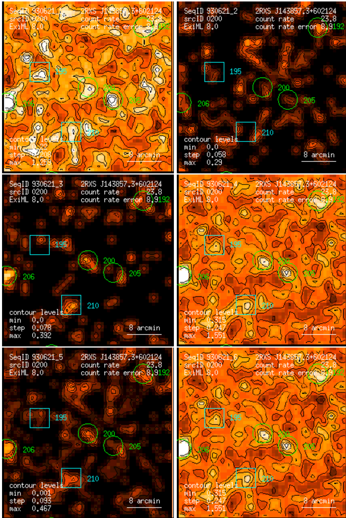
Figure 200: RASS 930621: detection 0200: band rate images, Gaussian filter: (1) PSPC channels 11 – 41, (2) 52 – 90, (3) 91 – 201, (4) 11 – 235, (5) 52 – 201, (6) 11 – 201. Broad band rates in counts/ks. Band rate contour levels in counts/ks/arcmin 2 .
