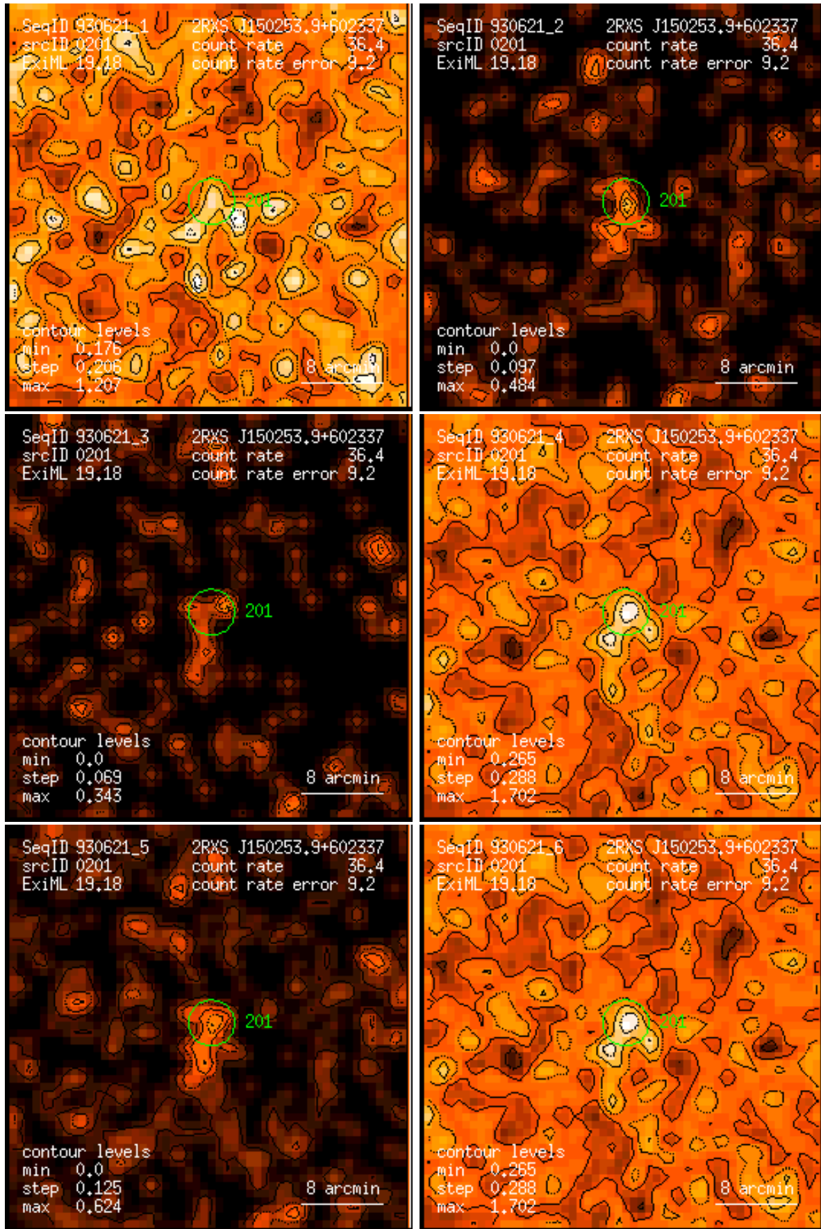
Figure 201: RASS 930621: detection 0201: band rate images, Gaussian filter: (1) PSPC channels 11 – 41, (2) 52 – 90, (3) 91 – 201, (4) 11 – 235, (5) 52 – 201, (6) 11 – 201. Broad band rates in counts/ks. Band rate contour levels in counts/ks/arcmin 2 .
