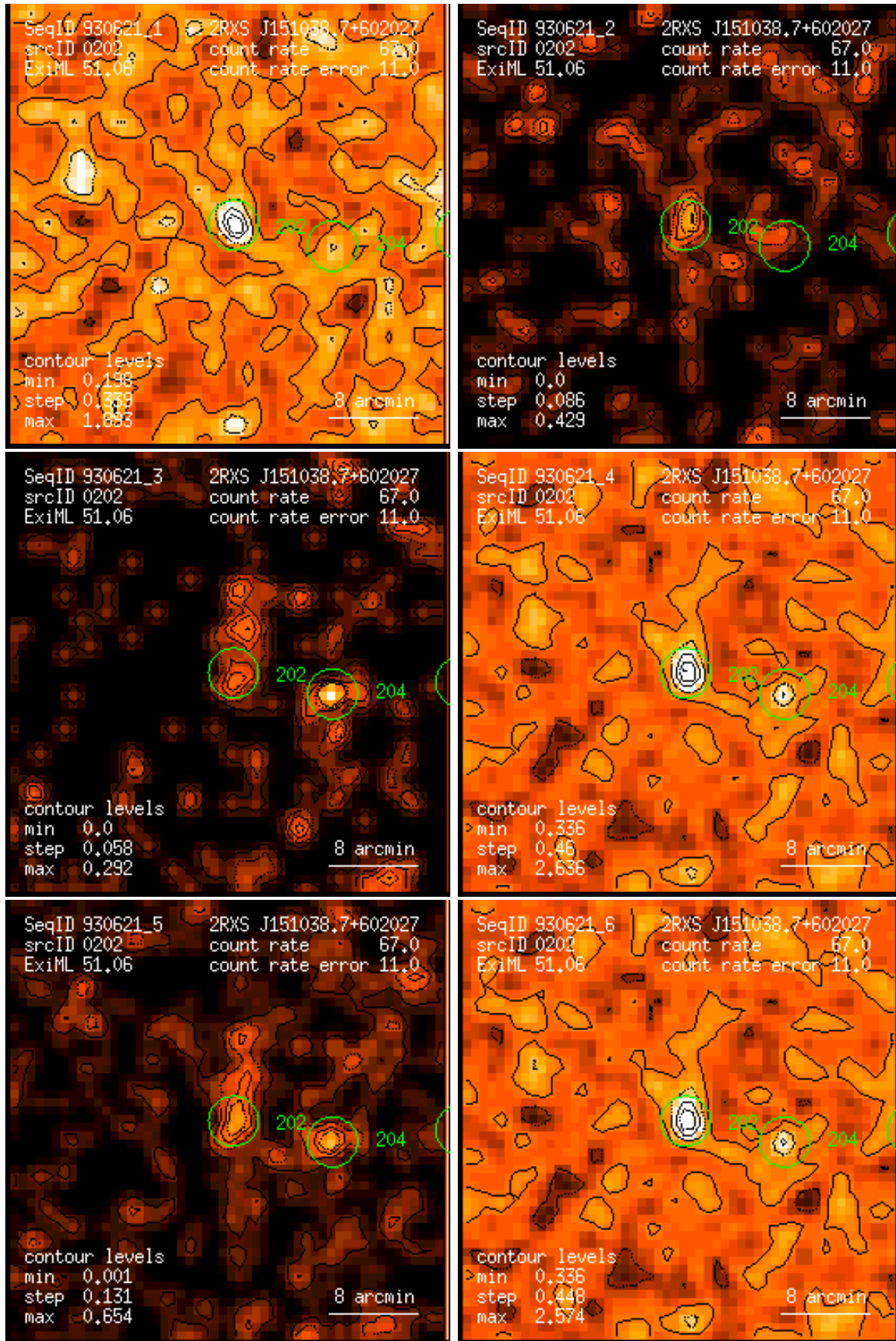
Figure 202: RASS 930621: detection 0202: band rate images, Gaussian filter: (1) PSPC channels 11 – 41, (2) 52 – 90, (3) 91 – 201, (4) 11 – 235, (5) 52 – 201, (6) 11 – 201. Broad band rates in counts/ks. Band rate contour levels in counts/ks/arcmin 2 .
