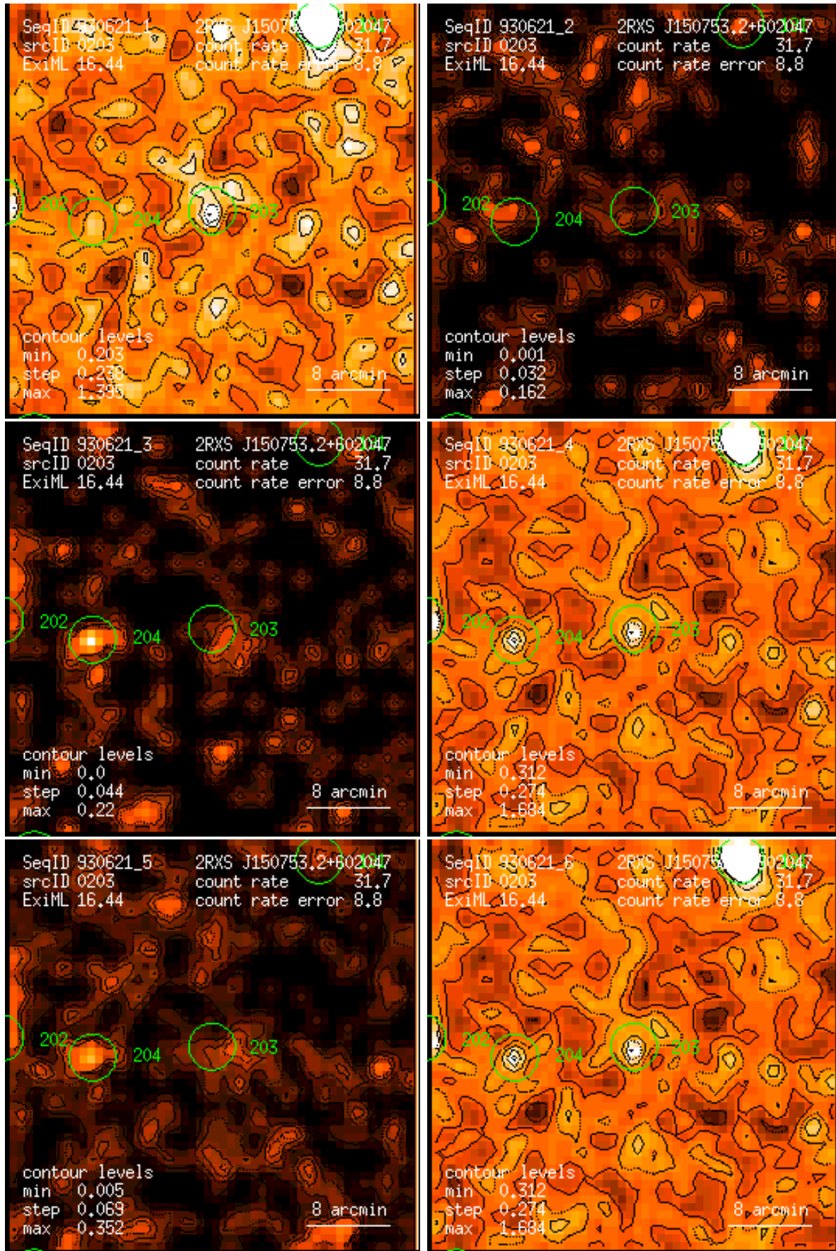
Figure 203: RASS 930621: detection 0203: band rate images, Gaussian filter: (1) PSPC channels 11 – 41, (2) 52 – 90, (3) 91 – 201, (4) 11 – 235, (5) 52 – 201, (6) 11 – 201. Broad band rates in counts/ks. Band rate contour levels in counts/ks/arcmin 2 .
