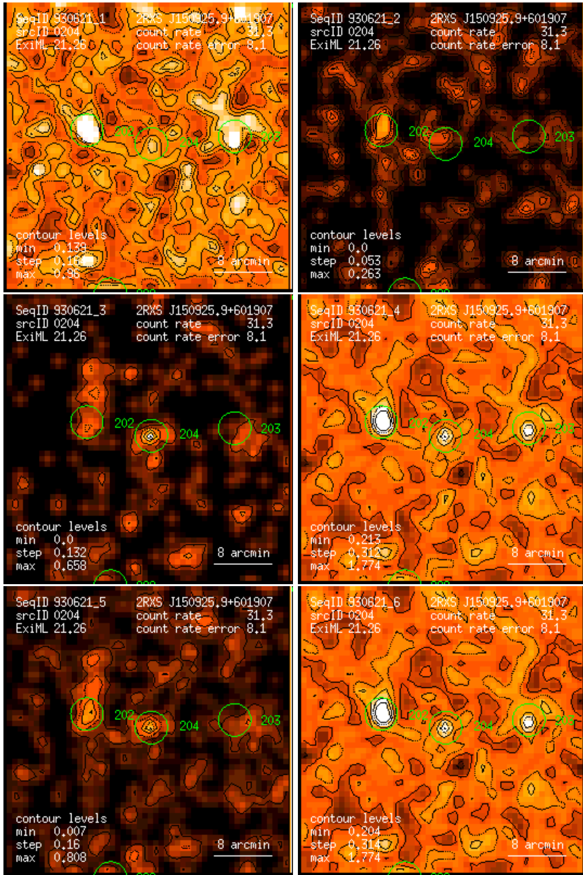
Figure 204: RASS 930621: detection 0204: band rate images, Gaussian filter: (1) PSPC channels 11 – 41, (2) 52 – 90, (3) 91 – 201, (4) 11 – 235, (5) 52 – 201, (6) 11 – 201. Broad band rates in counts/ks. Band rate contour levels in counts/ks/arcmin 2 .
