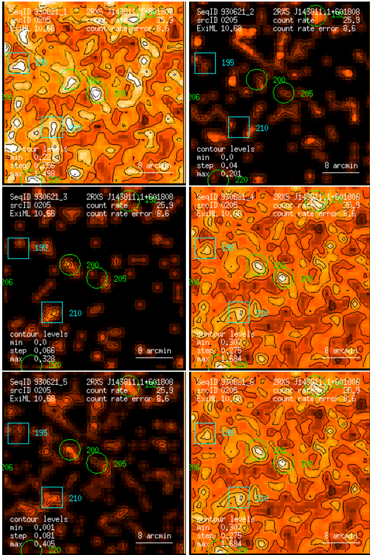
Figure 205: RASS 930621: detection 0205: band rate images, Gaussian filter: (1) PSPC channels 11 – 41, (2) 52 – 90, (3) 91 – 201, (4) 11 – 235, (5) 52 – 201, (6) 11 – 201. Broad band rates in counts/ks. Band rate contour levels in counts/ks/arcmin 2 .
