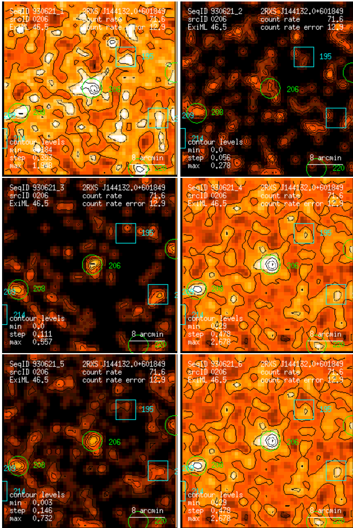
Figure 206: RASS 930621: detection 0206: band rate images, Gaussian filter: (1) PSPC channels 11 – 41, (2) 52 – 90, (3) 91 – 201, (4) 11 – 235, (5) 52 – 201, (6) 11 – 201. Broad band rates in counts/ks. Band rate contour levels in counts/ks/arcmin 2 .
