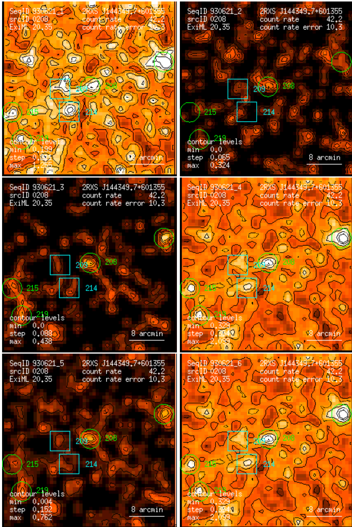
Figure 208: RASS 930621: detection 0208: band rate images, Gaussian filter: (1) PSPC channels 11 – 41, (2) 52 – 90, (3) 91 – 201, (4) 11 – 235, (5) 52 – 201, (6) 11 – 201. Broad band rates in counts/ks. Band rate contour levels in counts/ks/arcmin 2 .
