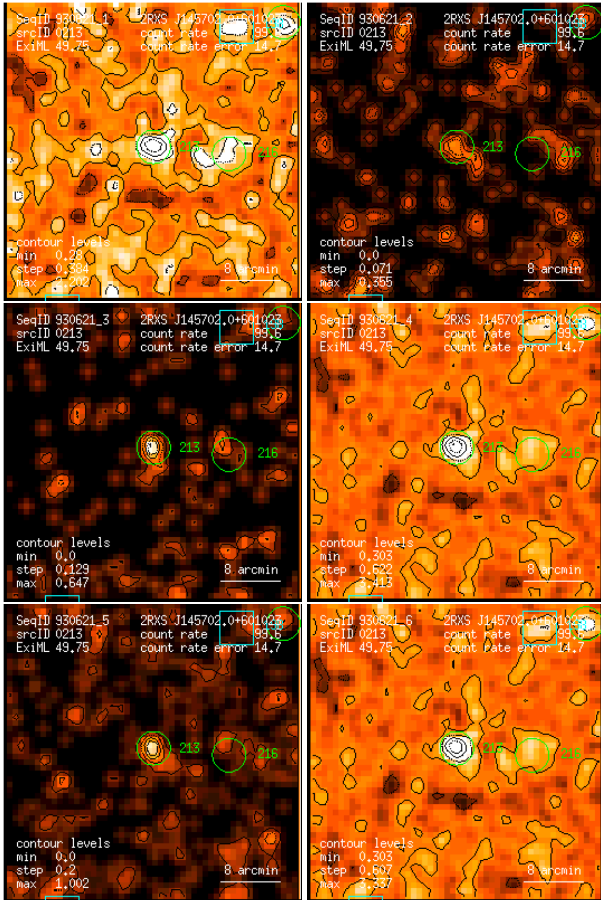
Figure 213: RASS 930621: detection 0213: band rate images, Gaussian filter: (1) PSPC channels 11 – 41, (2) 52 – 90, (3) 91 – 201, (4) 11 – 235, (5) 52 – 201, (6) 11 – 201. Broad band rates in counts/ks. Band rate contour levels in counts/ks/arcmin 2 .
