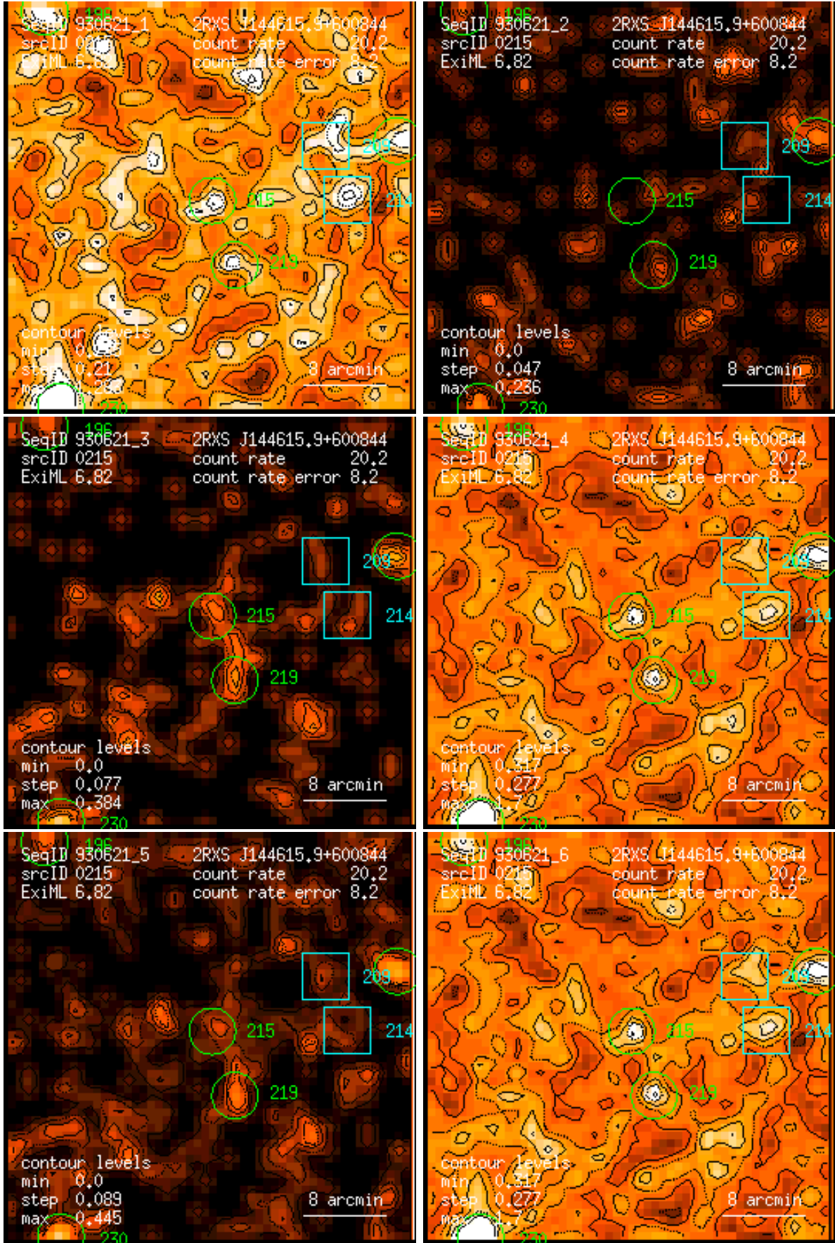
Figure 215: RASS 930621: detection 0215: band rate images, Gaussian filter: (1) PSPC channels 11 – 41, (2) 52 – 90, (3) 91 – 201, (4) 11 – 235, (5) 52 – 201, (6) 11 – 201. Broad band rates in counts/ks. Band rate contour levels in counts/ks/arcmin 2 .
