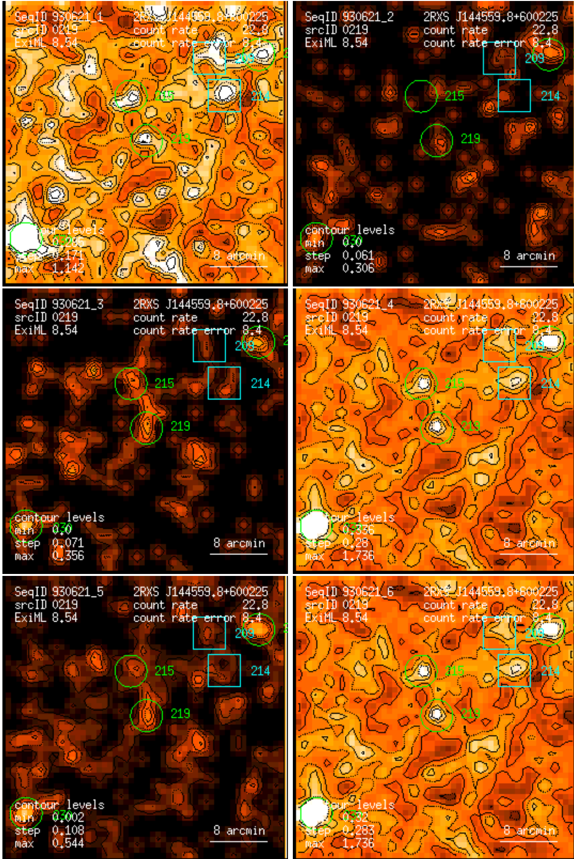
Figure 219: RASS 930621: detection 0219: band rate images, Gaussian filter: (1) PSPC channels 11 – 41, (2) 52 – 90, (3) 91 – 201, (4) 11 – 235, (5) 52 – 201, (6) 11 – 201. Broad band rates in counts/ks. Band rate contour levels in counts/ks/arcmin 2 .
