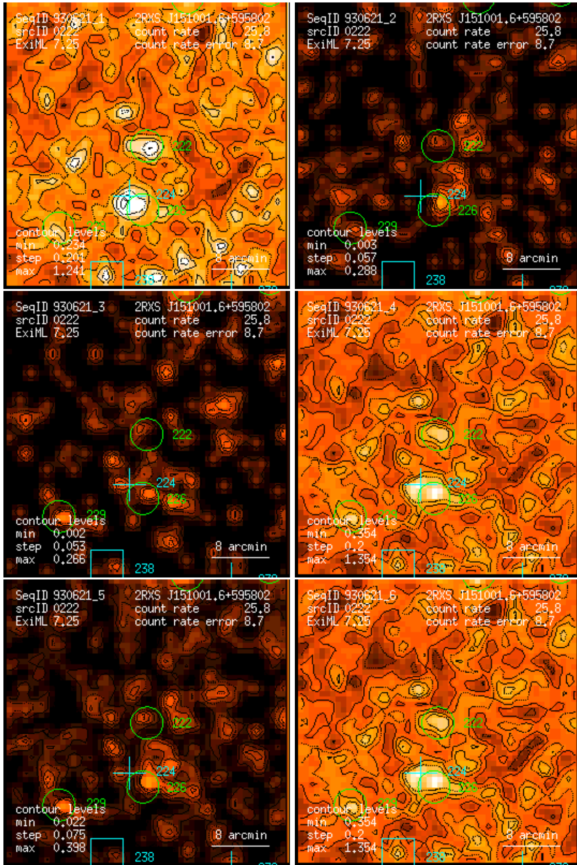
Figure 222: RASS 930621: detection 0222: band rate images, Gaussian filter: (1) PSPC channels 11 – 41, (2) 52 – 90, (3) 91 – 201, (4) 11 – 235, (5) 52 – 201, (6) 11 – 201. Broad band rates in counts/ks. Band rate contour levels in counts/ks/arcmin 2 .
