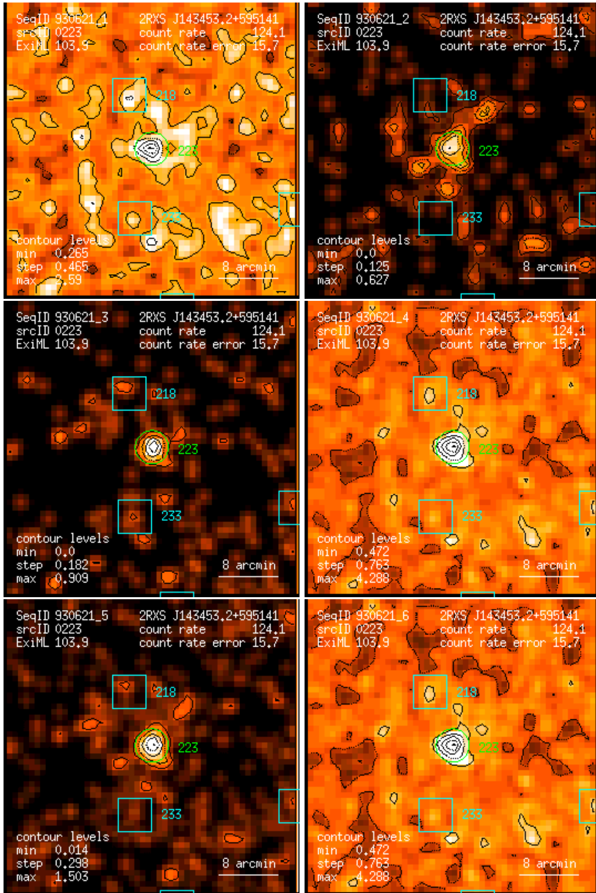
Figure 223: RASS 930621: detection 0223: band rate images, Gaussian filter: (1) PSPC channels 11 – 41, (2) 52 – 90, (3) 91 – 201, (4) 11 – 235, (5) 52 – 201, (6) 11 – 201. Broad band rates in counts/ks. Band rate contour levels in counts/ks/arcmin 2 .
