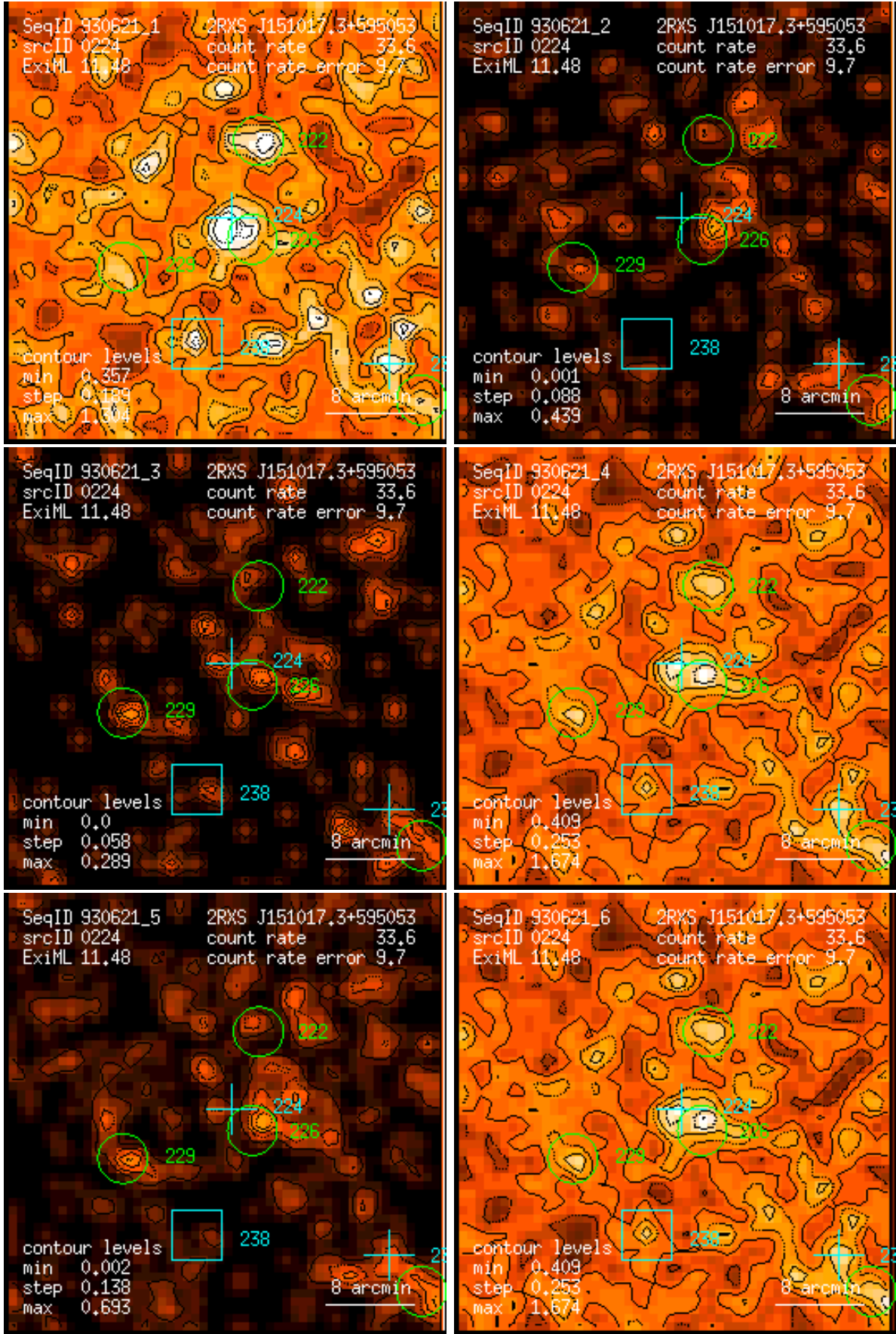
Figure 224: RASS 930621: detection 0224: band rate images, Gaussian filter: (1) PSPC channels 11 – 41, (2) 52 – 90, (3) 91 – 201, (4) 11 – 235, (5) 52 – 201, (6) 11 – 201. Broad band rates in counts/ks. Band rate contour levels in counts/ks/arcmin 2 .
