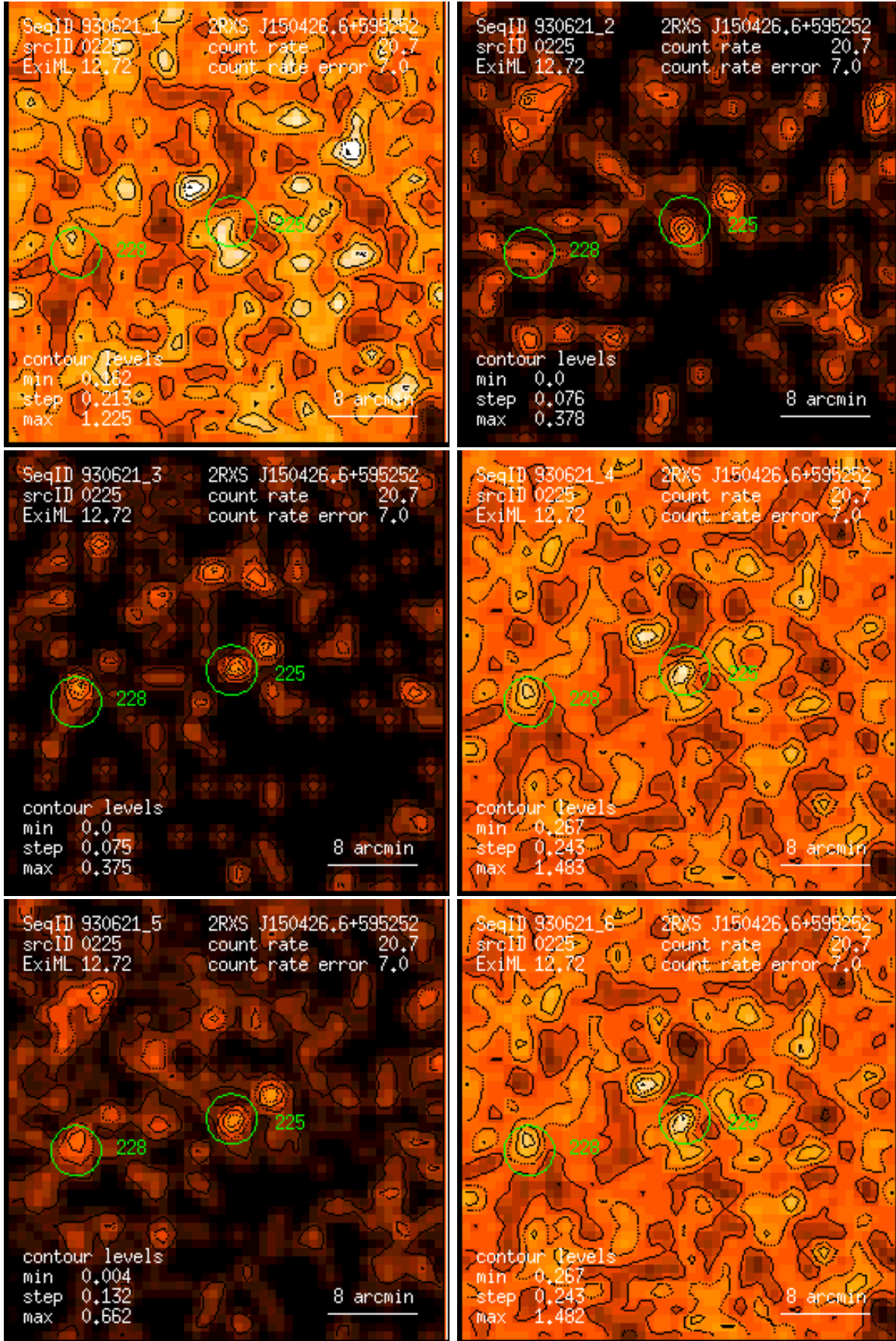
Figure 225: RASS 930621: detection 0225: band rate images, Gaussian filter: (1) PSPC channels 11 – 41, (2) 52 – 90, (3) 91 – 201, (4) 11 – 235, (5) 52 – 201, (6) 11 – 201. Broad band rates in counts/ks. Band rate contour levels in counts/ks/arcmin 2 .
