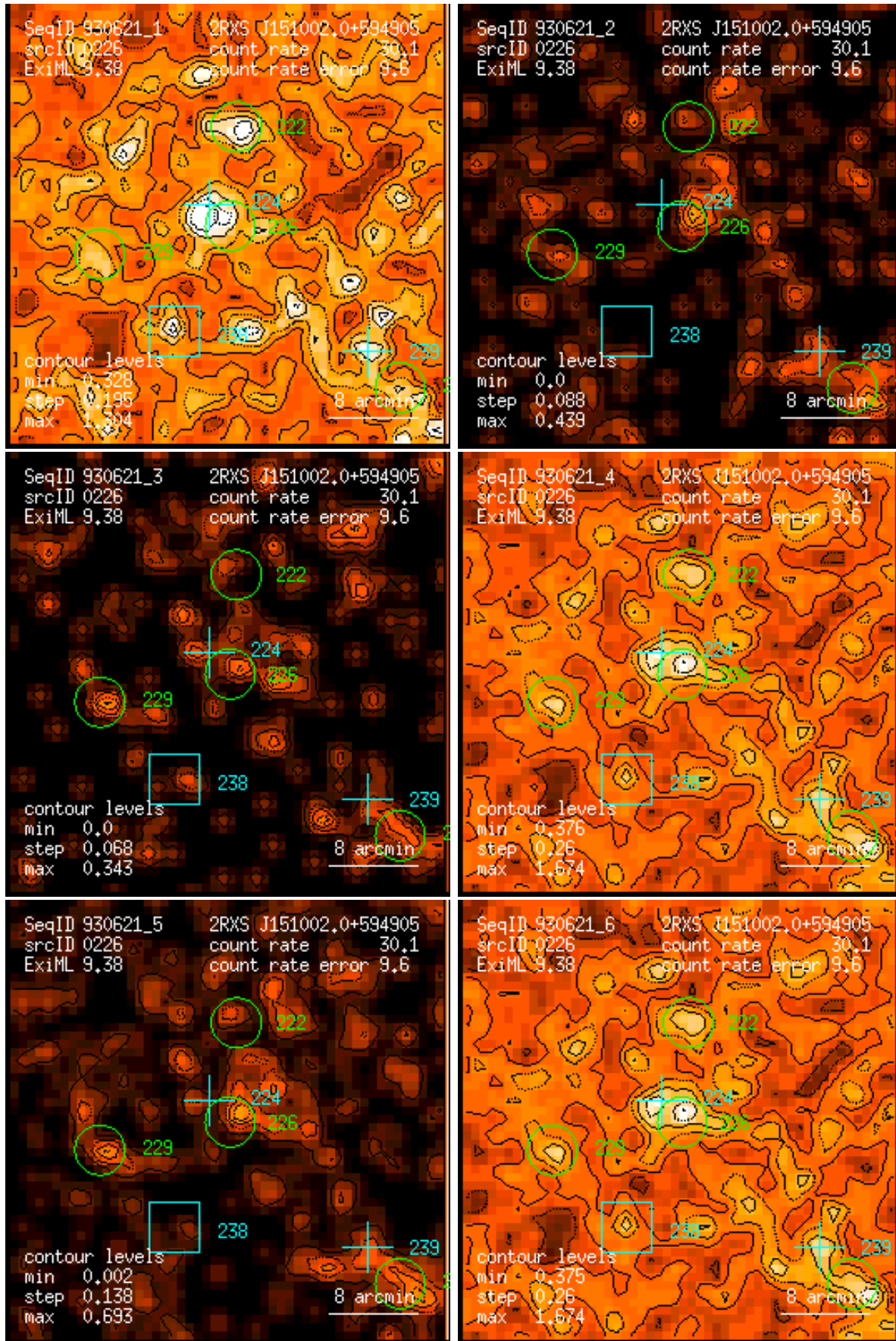
Figure 226: RASS 930621: detection 0226: band rate images, Gaussian filter: (1) PSPC channels 11 – 41, (2) 52 – 90, (3) 91 – 201, (4) 11 – 235, (5) 52 – 201, (6) 11 – 201. Broad band rates in counts/ks. Band rate contour levels in counts/ks/arcmin 2 .
