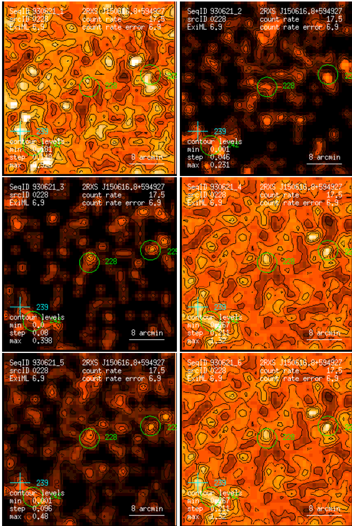
Figure 228: RASS 930621: detection 0228: band rate images, Gaussian filter: (1) PSPC channels 11 – 41, (2) 52 – 90, (3) 91 – 201, (4) 11 – 235, (5) 52 – 201, (6) 11 – 201. Broad band rates in counts/ks. Band rate contour levels in counts/ks/arcmin 2 .
