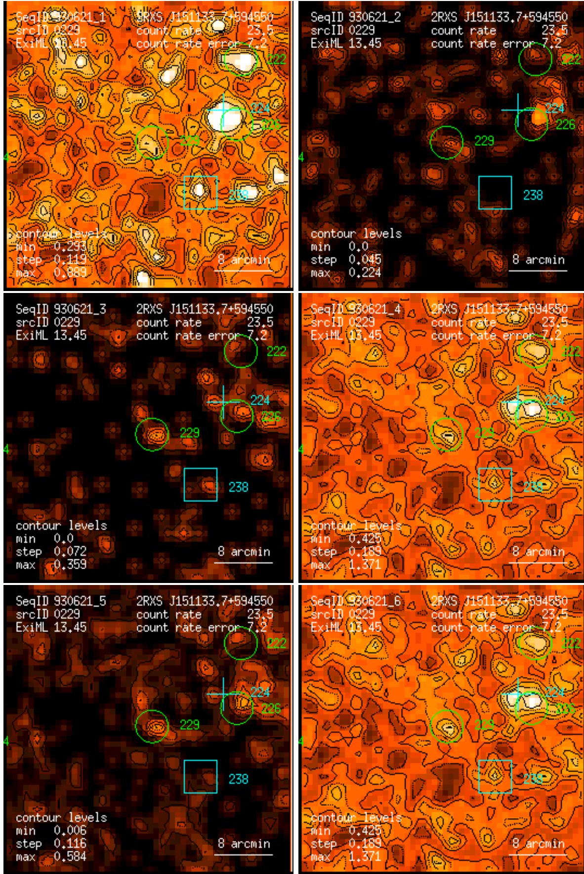
Figure 229: RASS 930621: detection 0229: band rate images, Gaussian filter: (1) PSPC channels 11 – 41, (2) 52 – 90, (3) 91 – 201, (4) 11 – 235, (5) 52 – 201, (6) 11 – 201. Broad band rates in counts/ks. Band rate contour levels in counts/ks/arcmin 2 .
