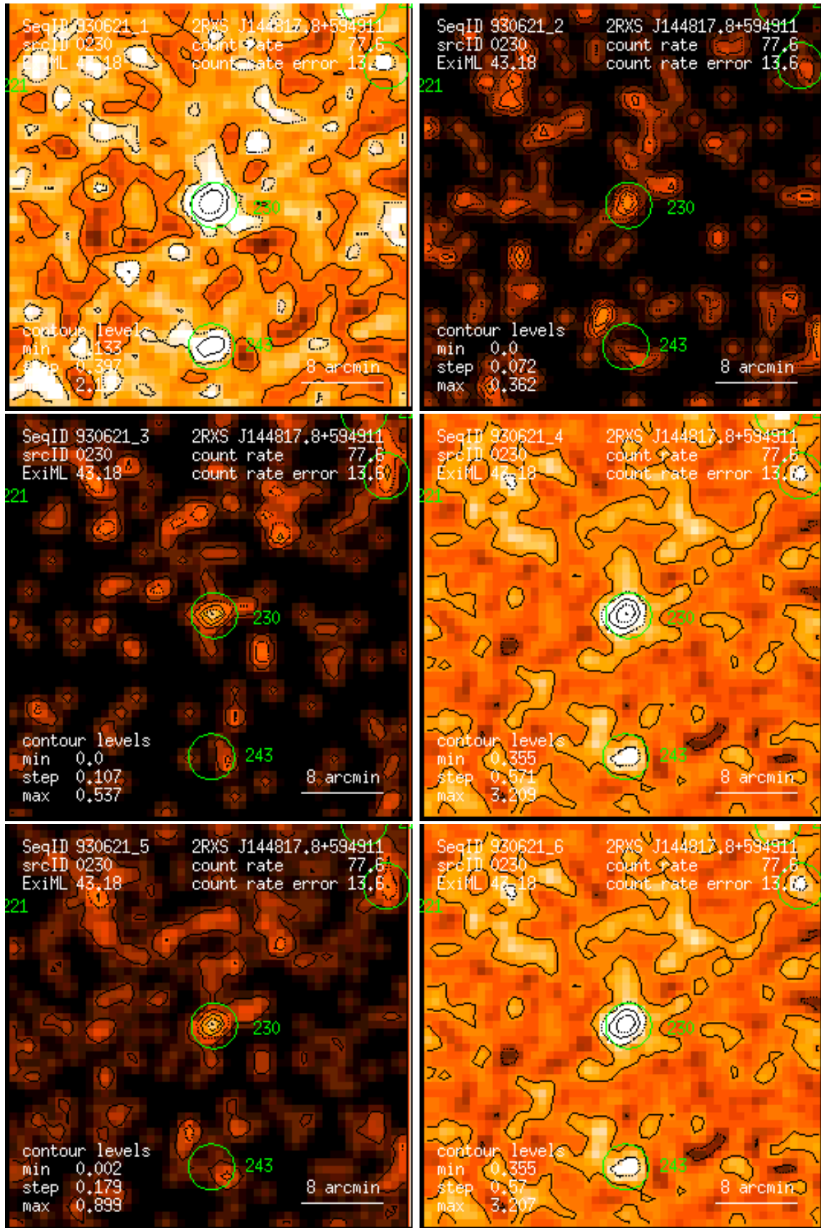
Figure 230: RASS 930621: detection 0230: band rate images, Gaussian filter: (1) PSPC channels 11 – 41, (2) 52 – 90, (3) 91 – 201, (4) 11 – 235, (5) 52 – 201, (6) 11 – 201. Broad band rates in counts/ks. Band rate contour levels in counts/ks/arcmin 2 .
