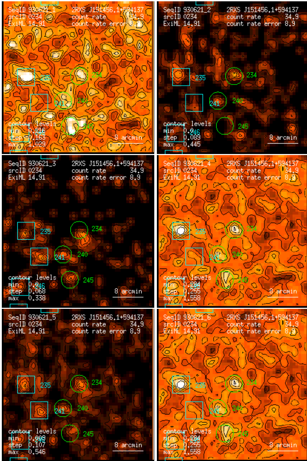
Figure 234: RASS 930621: detection 0234: band rate images, Gaussian filter: (1) PSPC channels 11 – 41, (2) 52 – 90, (3) 91 – 201, (4) 11 – 235, (5) 52 – 201, (6) 11 – 201. Broad band rates in counts/ks. Band rate contour levels in counts/ks/arcmin 2 .
