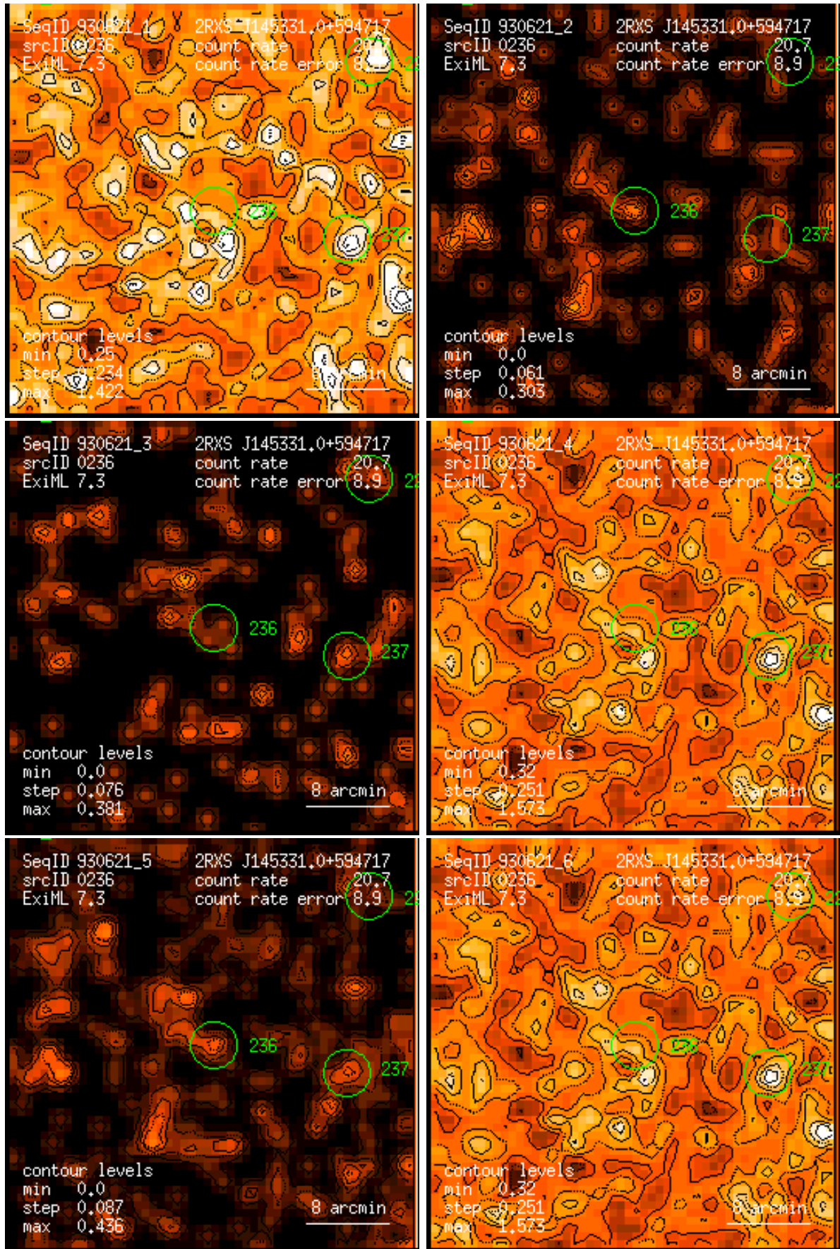
Figure 236: RASS 930621: detection 0236: band rate images, Gaussian filter: (1) PSPC channels 11 – 41, (2) 52 – 90, (3) 91 – 201, (4) 11 – 235, (5) 52 – 201, (6) 11 – 201. Broad band rates in counts/ks. Band rate contour levels in counts/ks/arcmin 2 .
