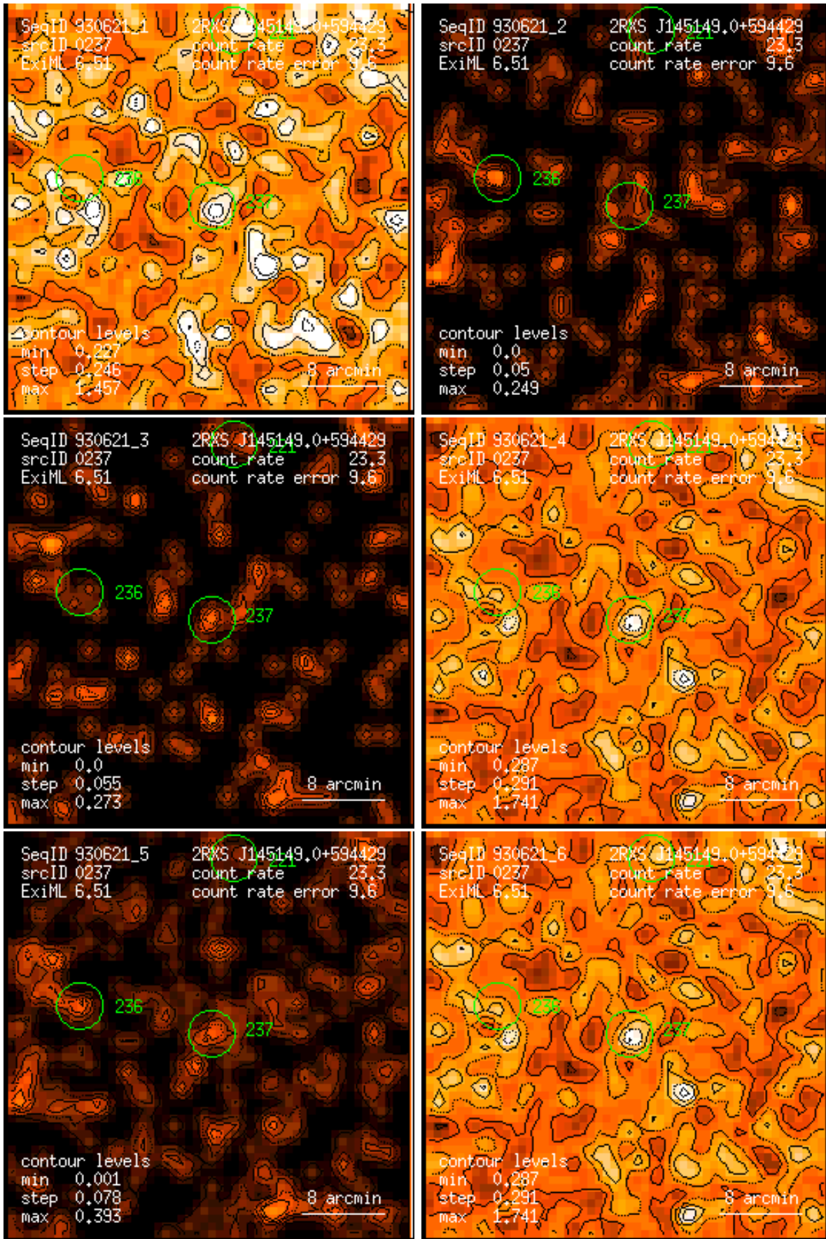
Figure 237: RASS 930621: detection 0237: band rate images, Gaussian filter: (1) PSPC channels 11 – 41, (2) 52 – 90, (3) 91 – 201, (4) 11 – 235, (5) 52 – 201, (6) 11 – 201. Broad band rates in counts/ks. Band rate contour levels in counts/ks/arcmin 2 .
