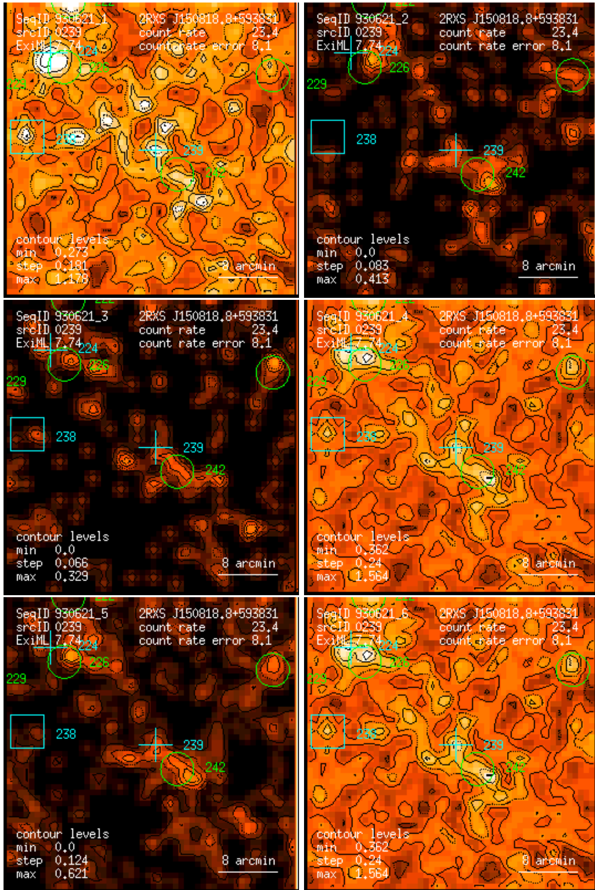
Figure 239: RASS 930621: detection 0239: band rate images, Gaussian filter: (1) PSPC channels 11 – 41, (2) 52 – 90, (3) 91 – 201, (4) 11 – 235, (5) 52 – 201, (6) 11 – 201. Broad band rates in counts/ks. Band rate contour levels in counts/ks/arcmin 2 .
