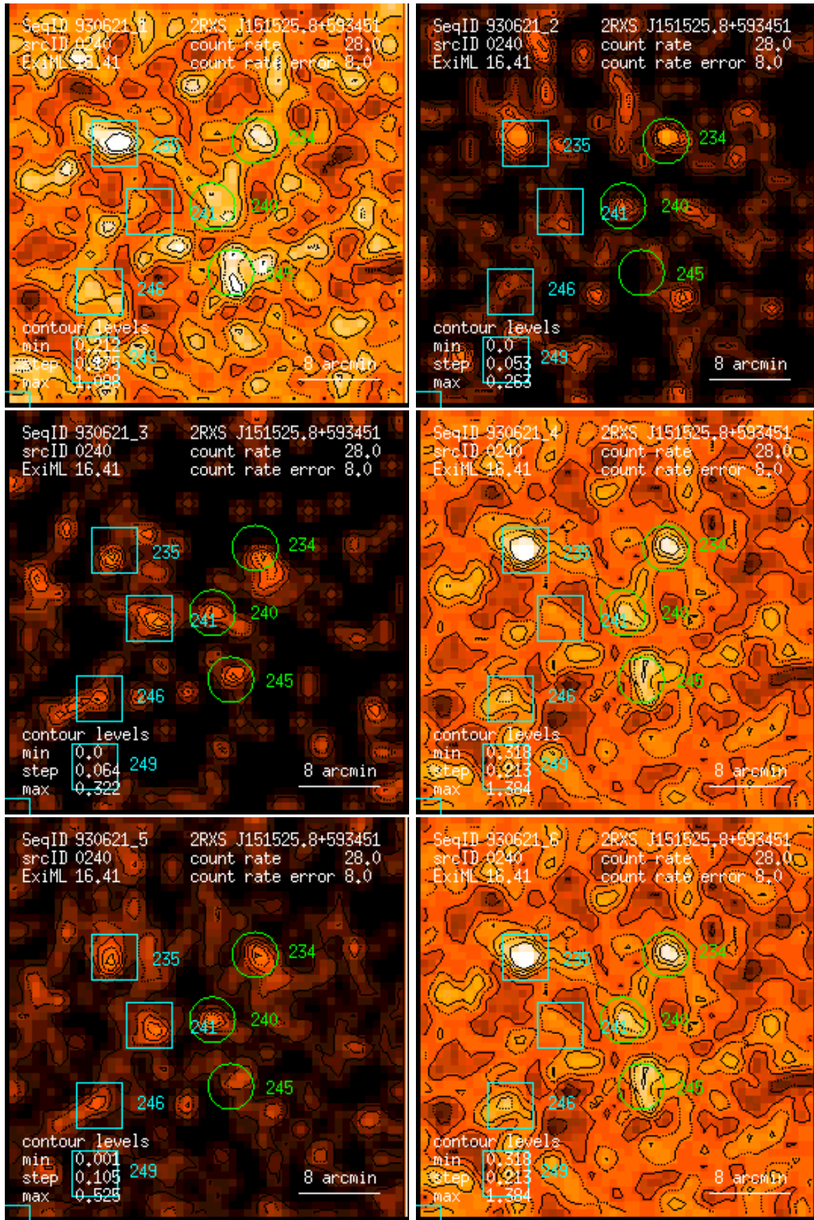
Figure 240: RASS 930621: detection 0240: band rate images, Gaussian filter: (1) PSPC channels 11 – 41, (2) 52 – 90, (3) 91 – 201, (4) 11 – 235, (5) 52 – 201, (6) 11 – 201. Broad band rates in counts/ks. Band rate contour levels in counts/ks/arcmin 2 .
