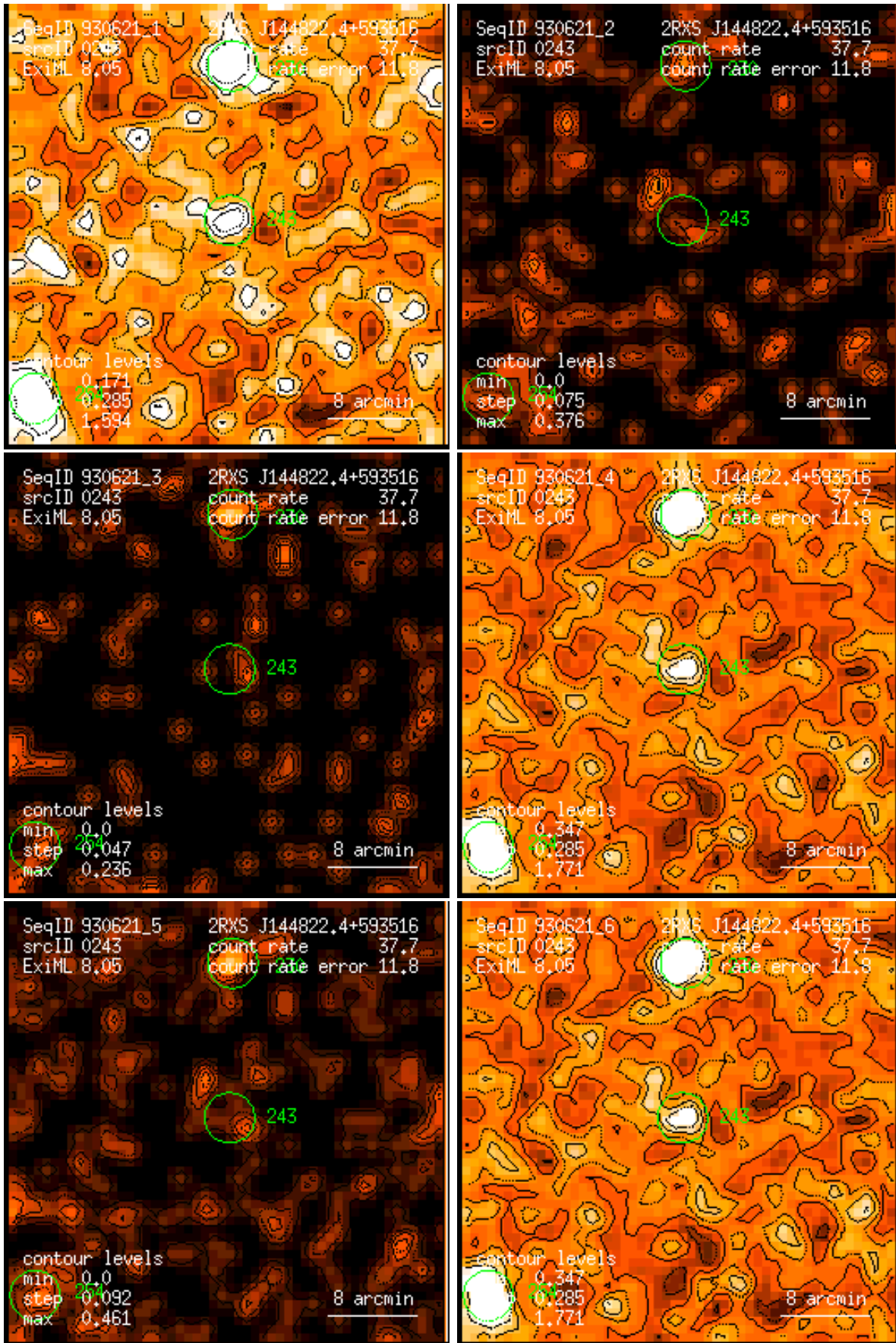
Figure 243: RASS 930621: detection 0243: band rate images, Gaussian filter: (1) PSPC channels 11 – 41, (2) 52 – 90, (3) 91 – 201, (4) 11 – 235, (5) 52 – 201, (6) 11 – 201. Broad band rates in counts/ks. Band rate contour levels in counts/ks/arcmin 2 .
