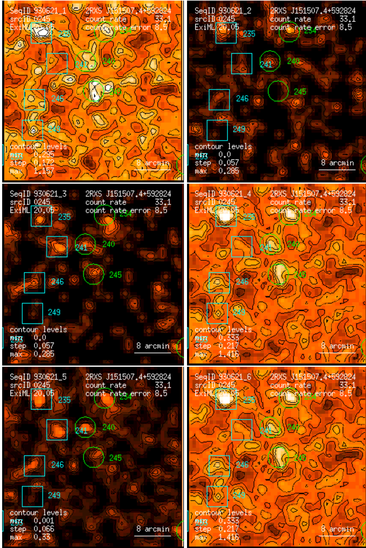
Figure 245: RASS 930621: detection 0245: band rate images, Gaussian filter: (1) PSPC channels 11 – 41, (2) 52 – 90, (3) 91 – 201, (4) 11 – 235, (5) 52 – 201, (6) 11 – 201. Broad band rates in counts/ks. Band rate contour levels in counts/ks/arcmin 2 .
