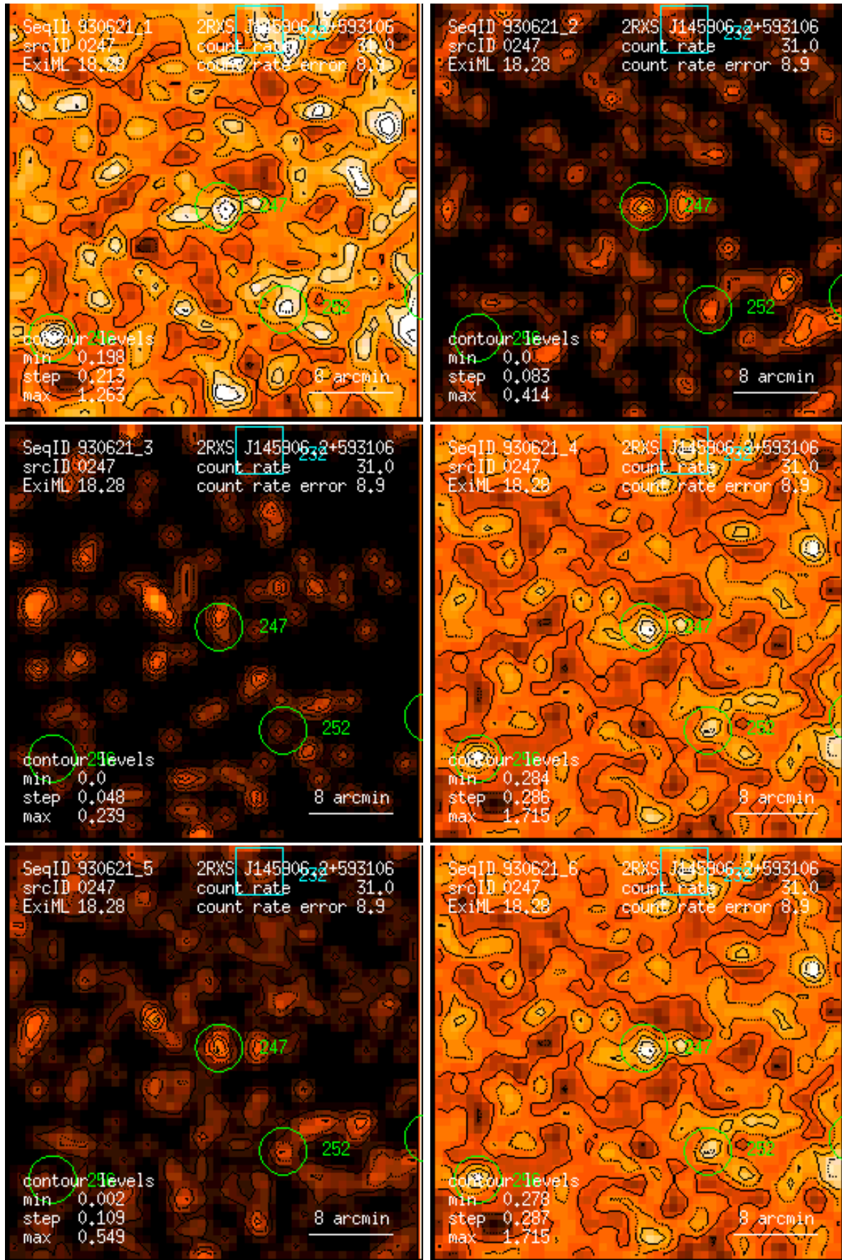
Figure 247: RASS 930621: detection 0247: band rate images, Gaussian filter: (1) PSPC channels 11 – 41, (2) 52 – 90, (3) 91 – 201, (4) 11 – 235, (5) 52 – 201, (6) 11 – 201. Broad band rates in counts/ks. Band rate contour levels in counts/ks/arcmin 2 .
