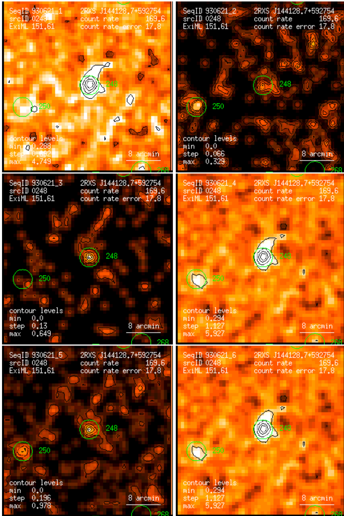
Figure 248: RASS 930621: detection 0248: band rate images, Gaussian filter: (1) PSPC channels 11 – 41, (2) 52 – 90, (3) 91 – 201, (4) 11 – 235, (5) 52 – 201, (6) 11 – 201. Broad band rates in counts/ks. Band rate contour levels in counts/ks/arcmin 2 .
