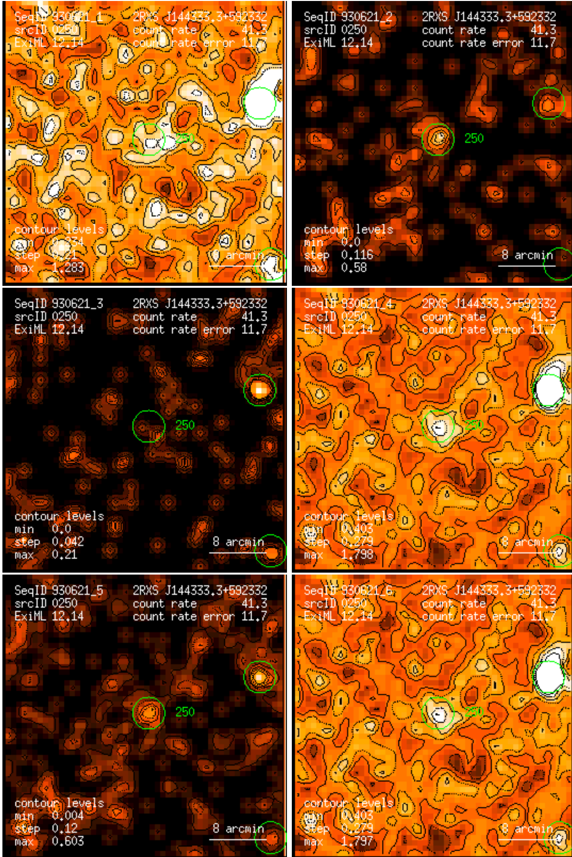
Figure 250: RASS 930621: detection 0250: band rate images, Gaussian filter: (1) PSPC channels 11 – 41, (2) 52 – 90, (3) 91 – 201, (4) 11 – 235, (5) 52 – 201, (6) 11 – 201. Broad band rates in counts/ks. Band rate contour levels in counts/ks/arcmin 2 .
