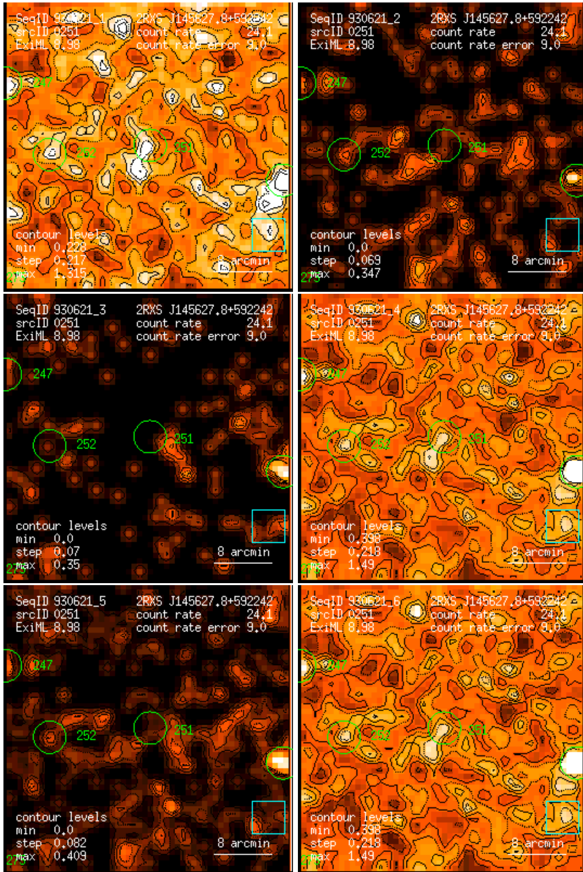
Figure 251: RASS 930621: detection 0251: band rate images, Gaussian filter: (1) PSPC channels 11 – 41, (2) 52 – 90, (3) 91 – 201, (4) 11 – 235, (5) 52 – 201, (6) 11 – 201. Broad band rates in counts/ks. Band rate contour levels in counts/ks/arcmin 2 .
