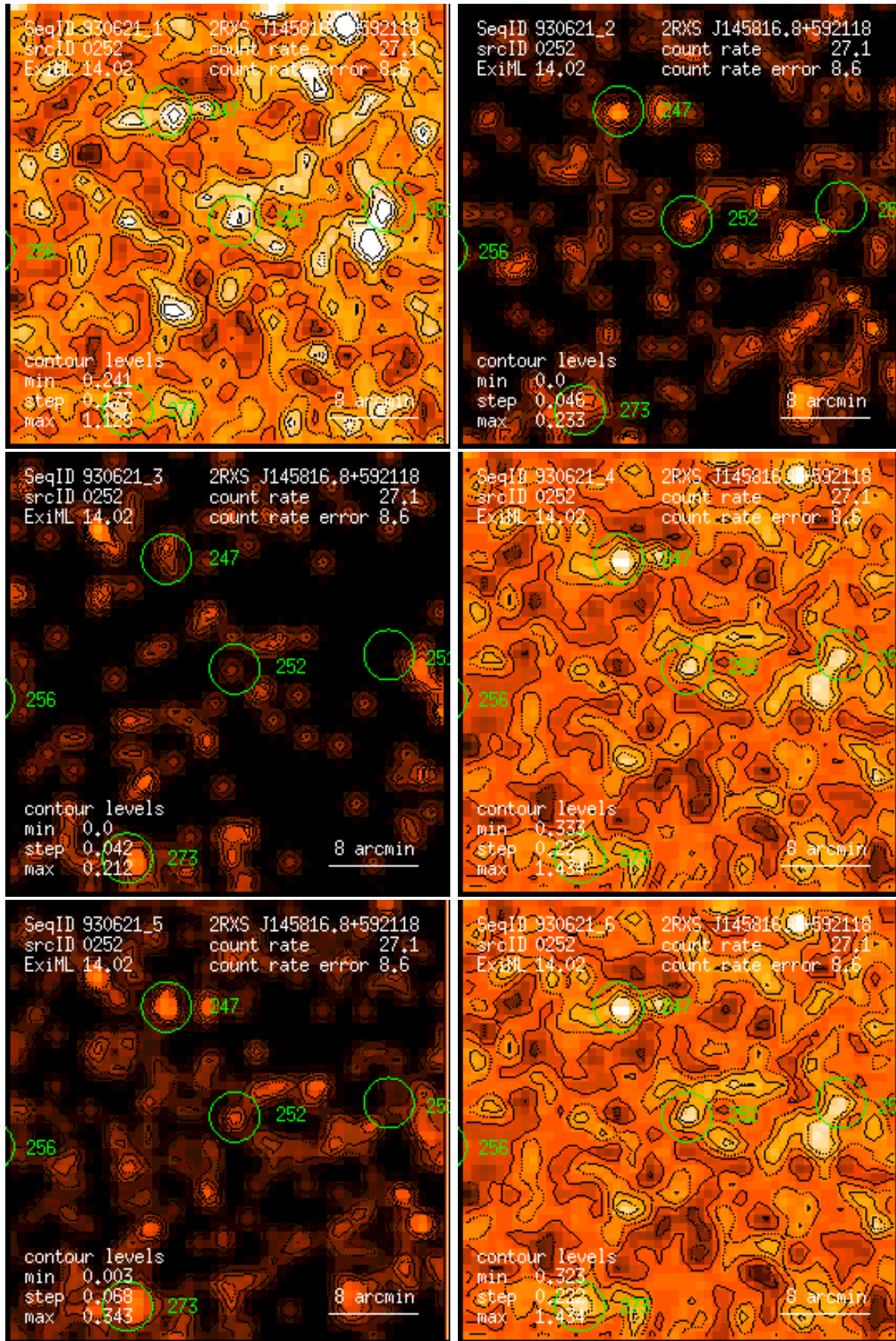
Figure 252: RASS 930621: detection 0252: band rate images, Gaussian filter: (1) PSPC channels 11 – 41, (2) 52 – 90, (3) 91 – 201, (4) 11 – 235, (5) 52 – 201, (6) 11 – 201. Broad band rates in counts/ks. Band rate contour levels in counts/ks/arcmin 2 .
