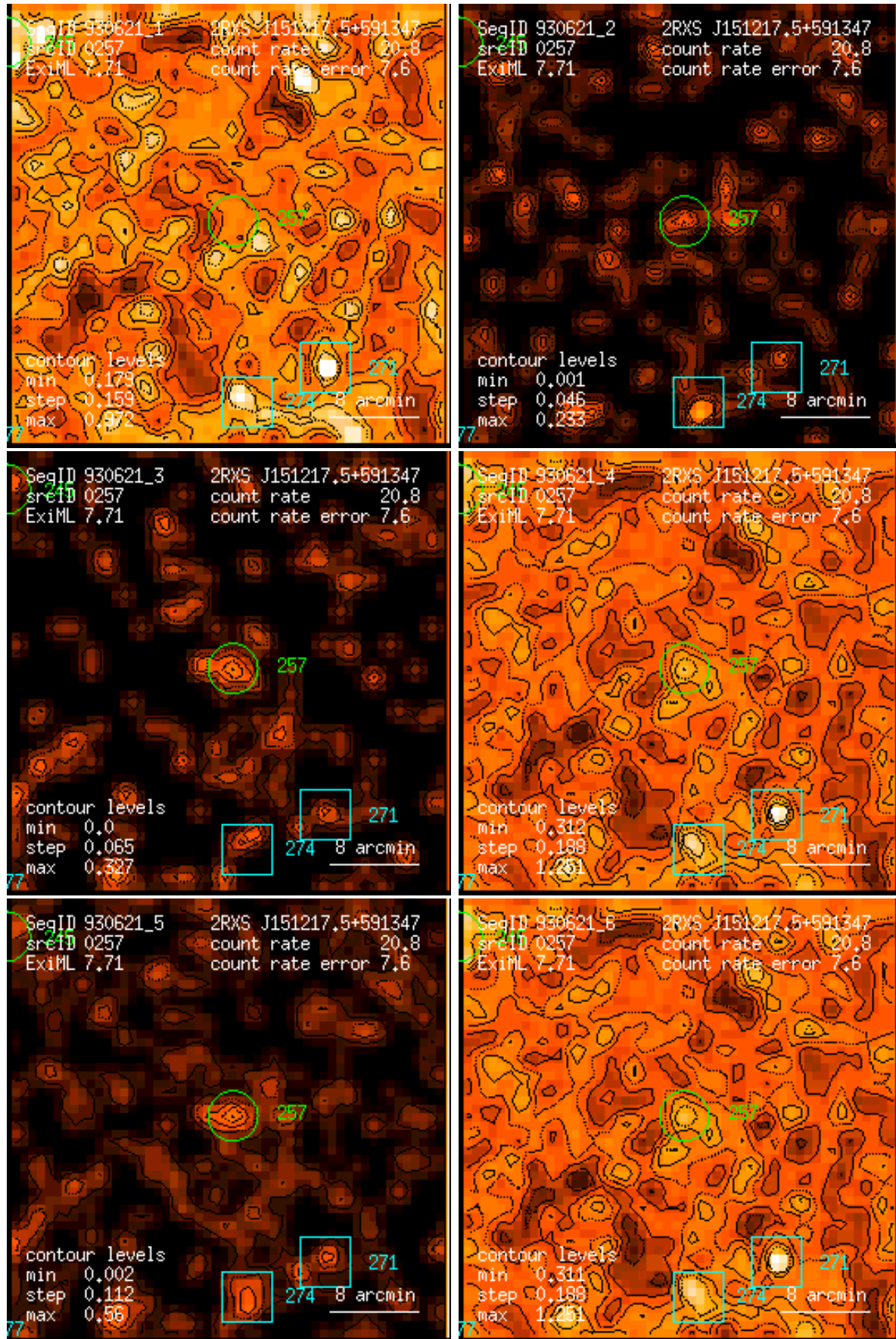
Figure 257: RASS 930621: detection 0257: band rate images, Gaussian filter: (1) PSPC channels 11 – 41, (2) 52 – 90, (3) 91 – 201, (4) 11 – 235, (5) 52 – 201, (6) 11 – 201. Broad band rates in counts/ks. Band rate contour levels in counts/ks/arcmin 2 .
