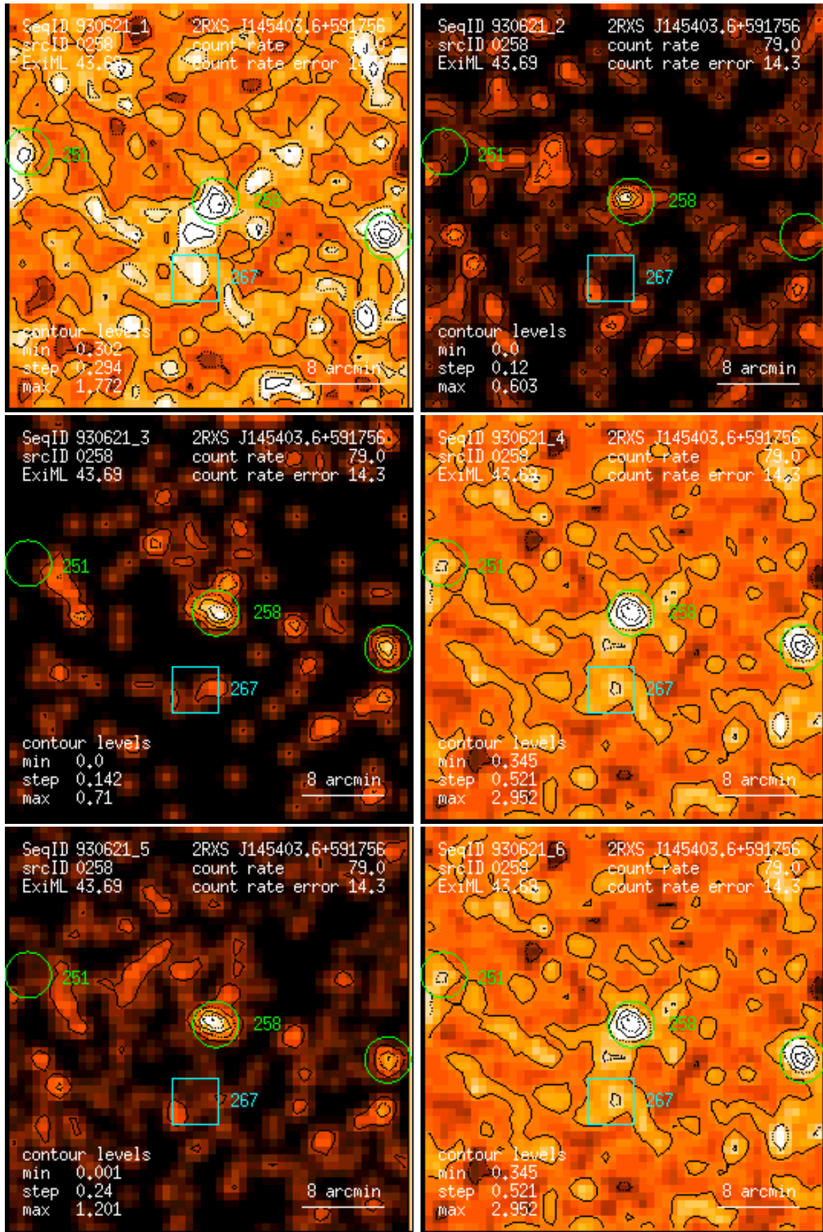
Figure 258: RASS 930621: detection 0258: band rate images, Gaussian filter: (1) PSPC channels 11 – 41, (2) 52 – 90, (3) 91 – 201, (4) 11 – 235, (5) 52 – 201, (6) 11 – 201. Broad band rates in counts/ks. Band rate contour levels in counts/ks/arcmin 2 .
