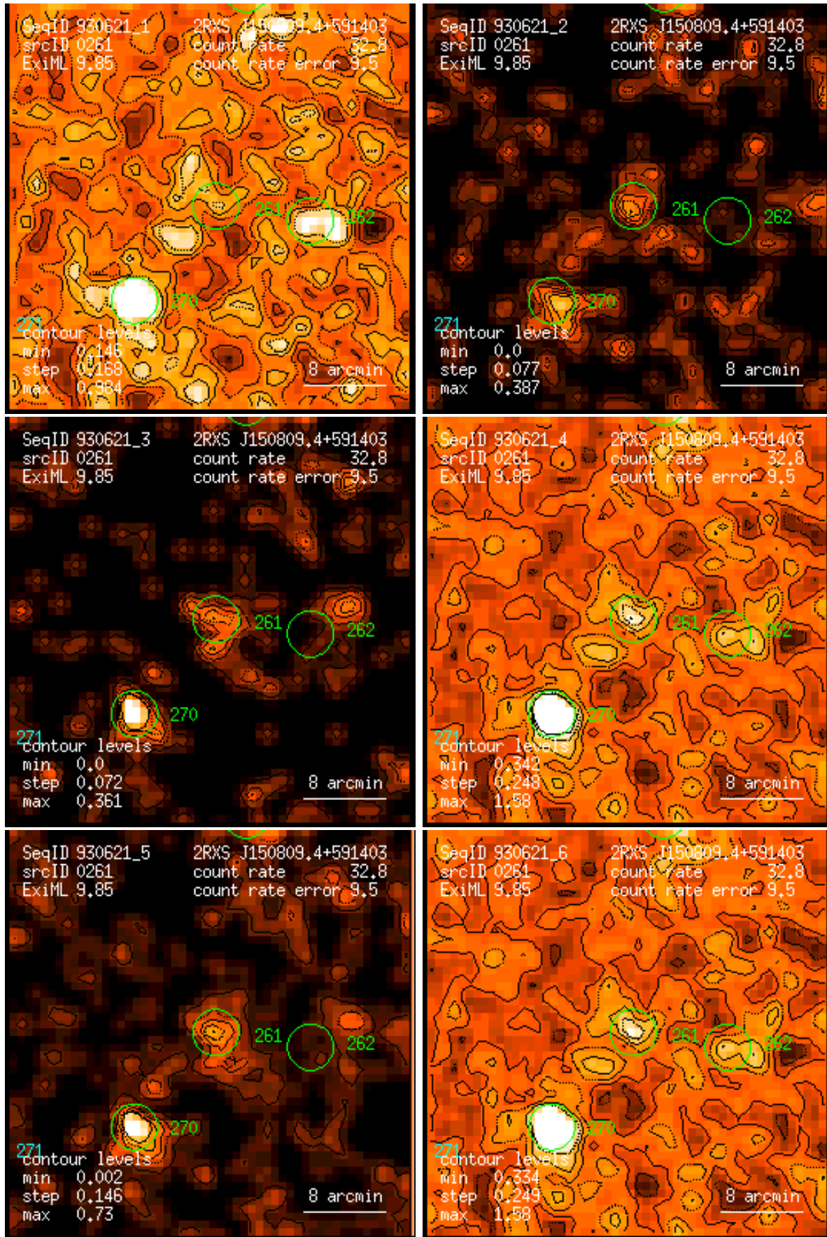
Figure 261: RASS 930621: detection 0261: band rate images, Gaussian filter: (1) PSPC channels 11 – 41, (2) 52 – 90, (3) 91 – 201, (4) 11 – 235, (5) 52 – 201, (6) 11 – 201. Broad band rates in counts/ks. Band rate contour levels in counts/ks/arcmin 2 .
