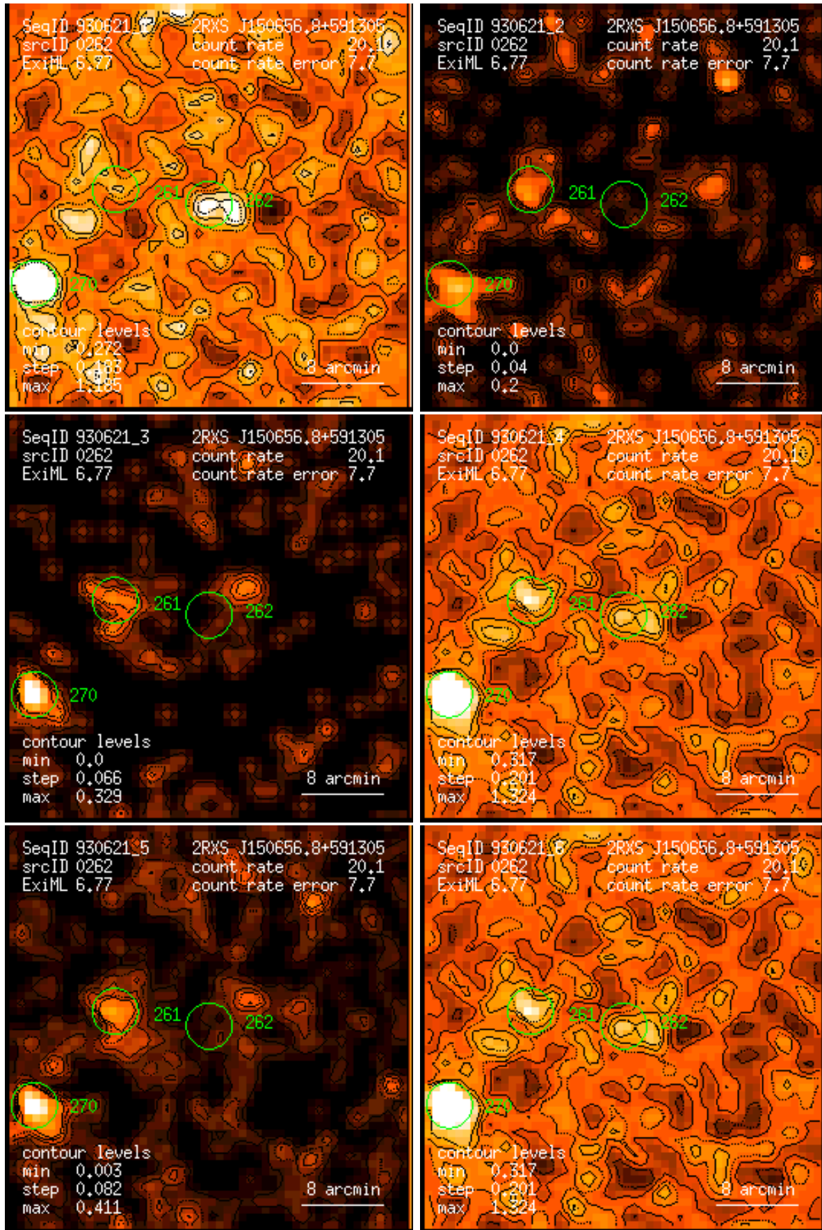
Figure 262: RASS 930621: detection 0262: band rate images, Gaussian filter: (1) PSPC channels 11 – 41, (2) 52 – 90, (3) 91 – 201, (4) 11 – 235, (5) 52 – 201, (6) 11 – 201. Broad band rates in counts/ks. Band rate contour levels in counts/ks/arcmin 2 .
