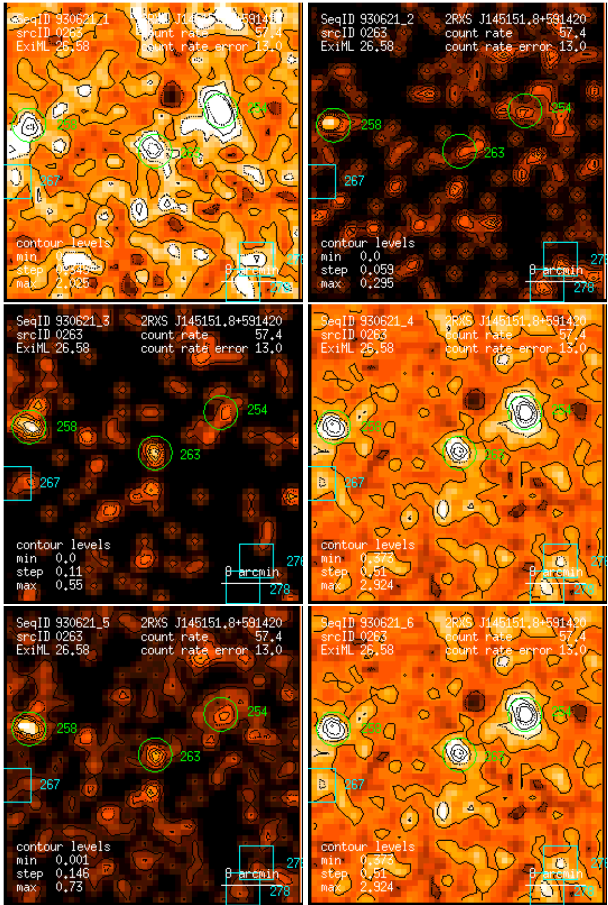
Figure 263: RASS 930621: detection 0263: band rate images, Gaussian filter: (1) PSPC channels 11 – 41, (2) 52 – 90, (3) 91 – 201, (4) 11 – 235, (5) 52 – 201, (6) 11 – 201. Broad band rates in counts/ks. Band rate contour levels in counts/ks/arcmin 2 .
