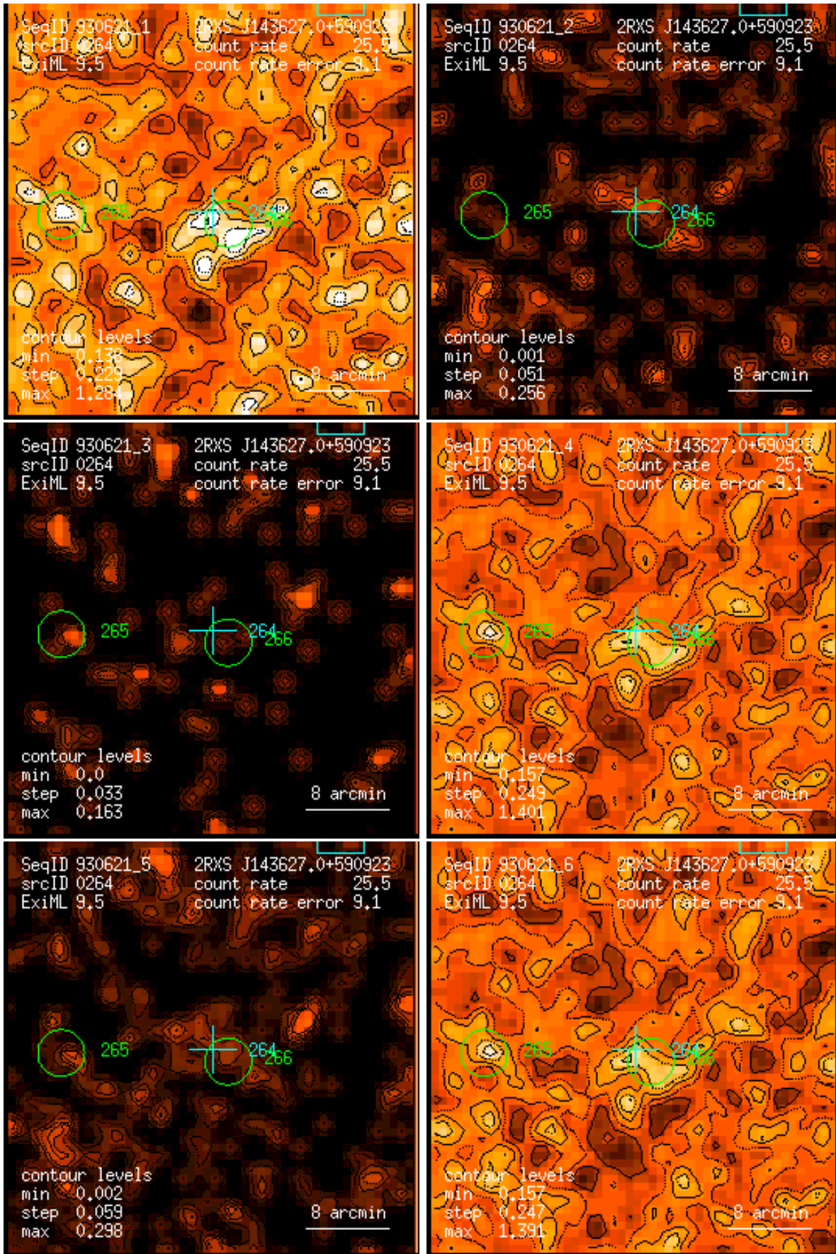
Figure 264: RASS 930621: detection 0264: band rate images, Gaussian filter: (1) PSPC channels 11 – 41, (2) 52 – 90, (3) 91 – 201, (4) 11 – 235, (5) 52 – 201, (6) 11 – 201. Broad band rates in counts/ks. Band rate contour levels in counts/ks/arcmin 2 .
