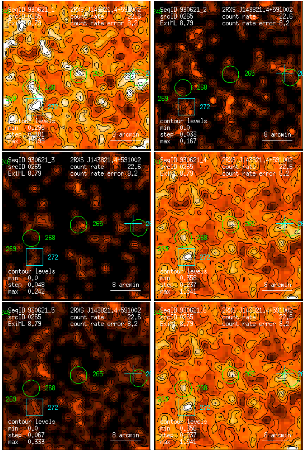
Figure 265: RASS 930621: detection 0265: band rate images, Gaussian filter: (1) PSPC channels 11 – 41, (2) 52 – 90, (3) 91 – 201, (4) 11 – 235, (5) 52 – 201, (6) 11 – 201. Broad band rates in counts/ks. Band rate contour levels in counts/ks/arcmin 2 .
