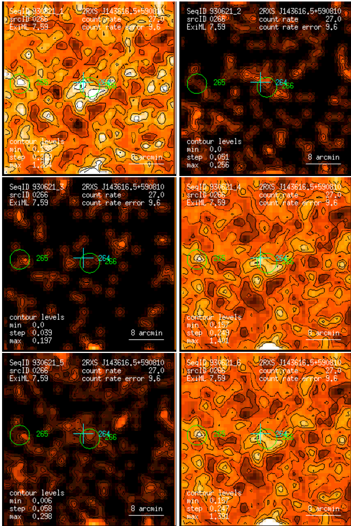
Figure 266: RASS 930621: detection 0266: band rate images, Gaussian filter: (1) PSPC channels 11 – 41, (2) 52 – 90, (3) 91 – 201, (4) 11 – 235, (5) 52 – 201, (6) 11 – 201. Broad band rates in counts/ks. Band rate contour levels in counts/ks/arcmin 2 .
