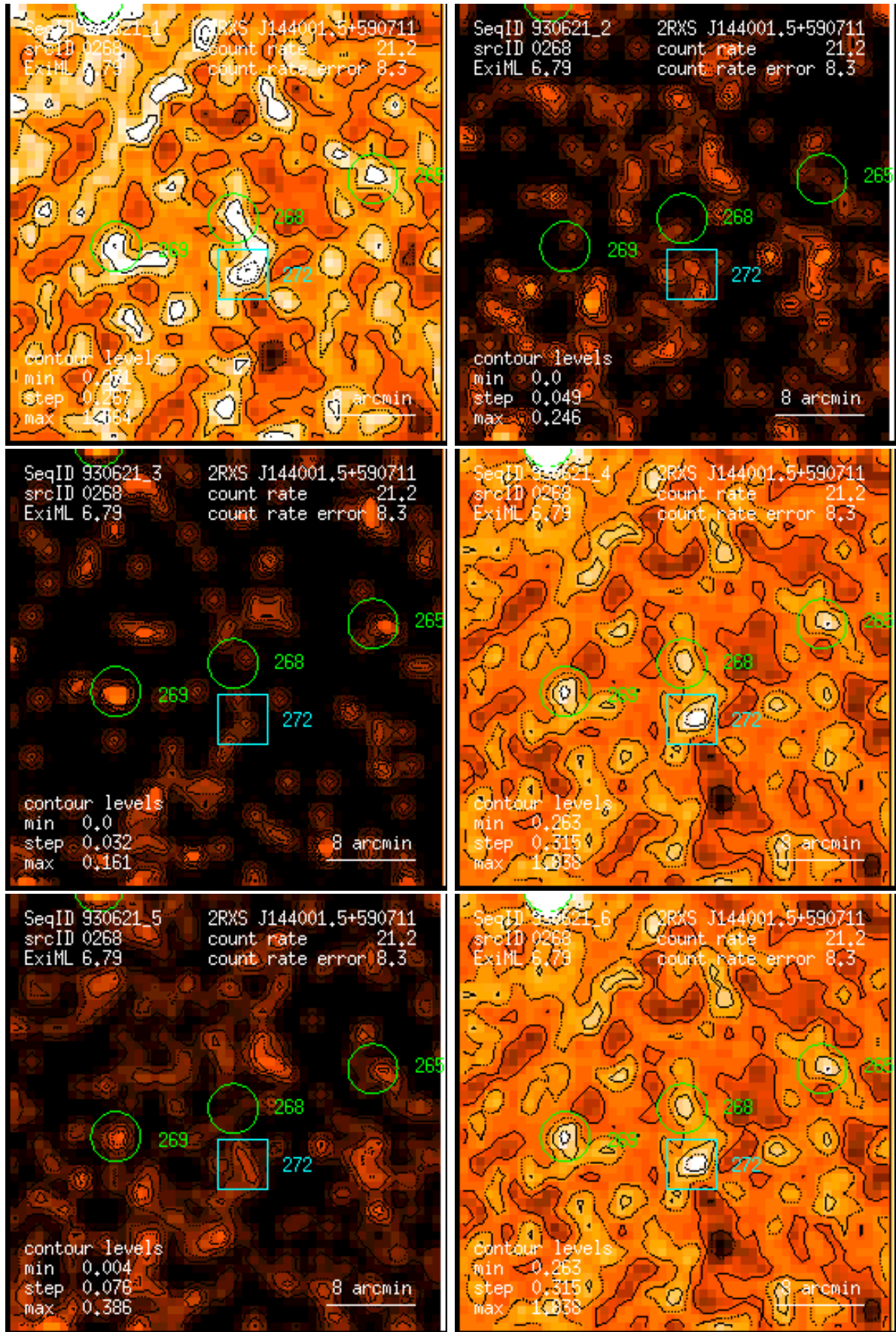
Figure 268: RASS 930621: detection 0268: band rate images, Gaussian filter: (1) PSPC channels 11 – 41, (2) 52 – 90, (3) 91 – 201, (4) 11 – 235, (5) 52 – 201, (6) 11 – 201. Broad band rates in counts/ks. Band rate contour levels in counts/ks/arcmin 2 .
