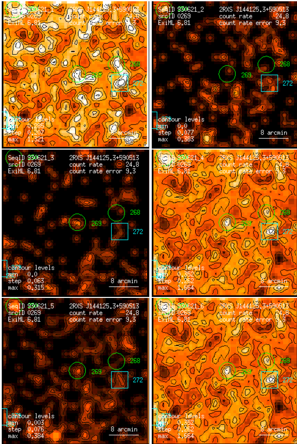
Figure 269: RASS 930621: detection 0269: band rate images, Gaussian filter: (1) PSPC channels 11 – 41, (2) 52 – 90, (3) 91 – 201, (4) 11 – 235, (5) 52 – 201, (6) 11 – 201. Broad band rates in counts/ks. Band rate contour levels in counts/ks/arcmin 2 .
