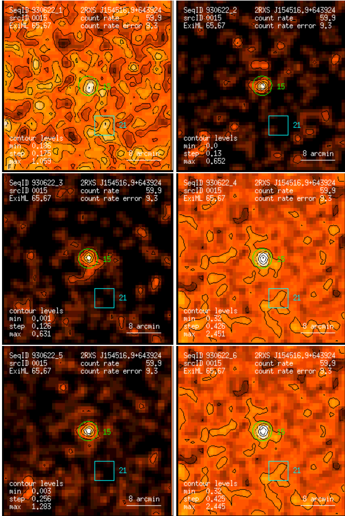
Figure 15: RASS 930622: detection 0015: band rate images, Gaussian filter: (1) PSPC channels 11 – 41, (2) 52 – 90, (3) 91 – 201, (4) 11 – 235, (5) 52 – 201, (6) 11 – 201. Broad band rates in counts/ks. Band rate contour levels in counts/ks/arcmin 2 .
