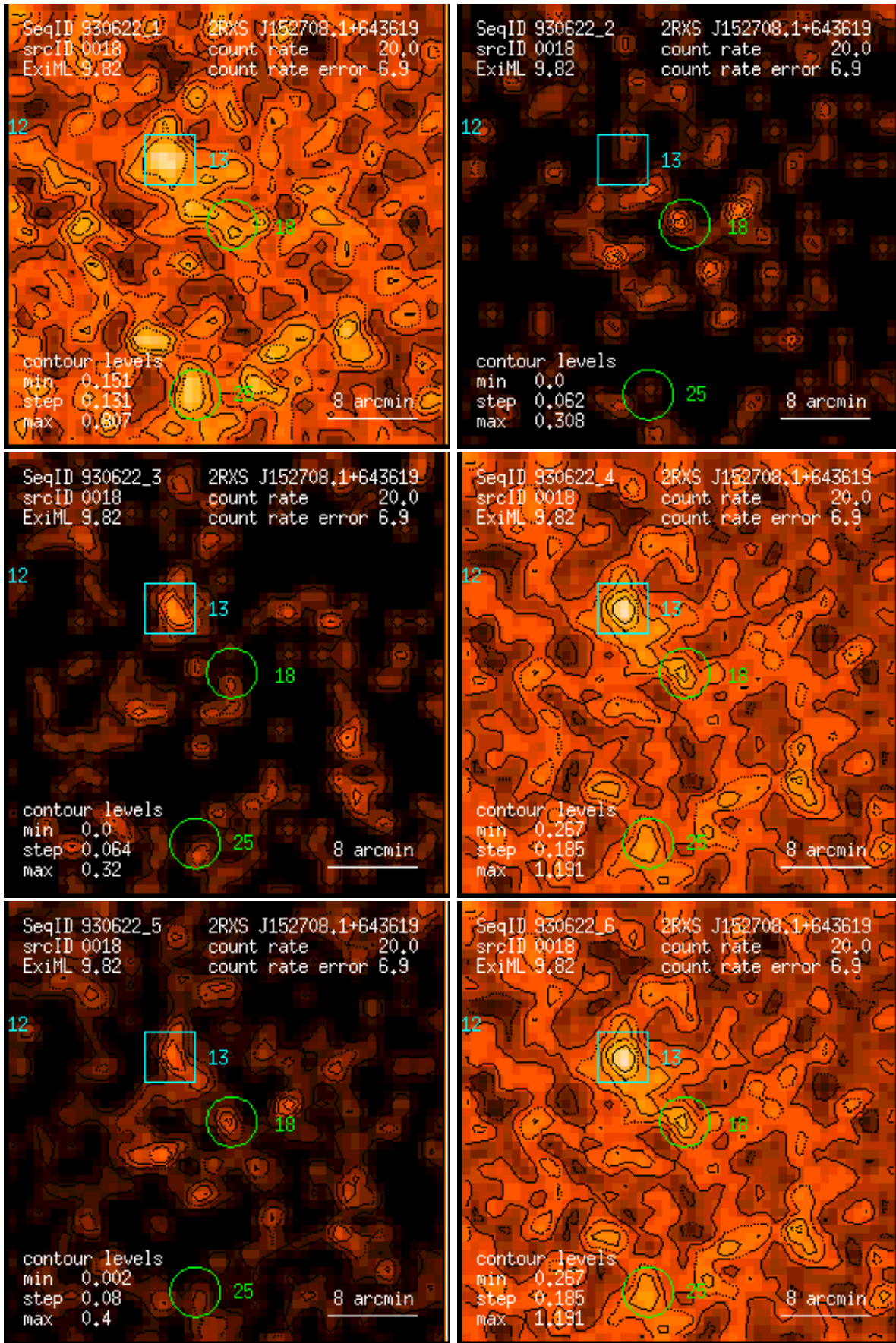
Figure 18: RASS 930622: detection 0018: band rate images, Gaussian filter: (1) PSPC channels 11 – 41, (2) 52 – 90, (3) 91 – 201, (4) 11 – 235, (5) 52 – 201, (6) 11 – 201. Broad band rates in counts/ks. Band rate contour levels in counts/ks/arcmin 2 .
