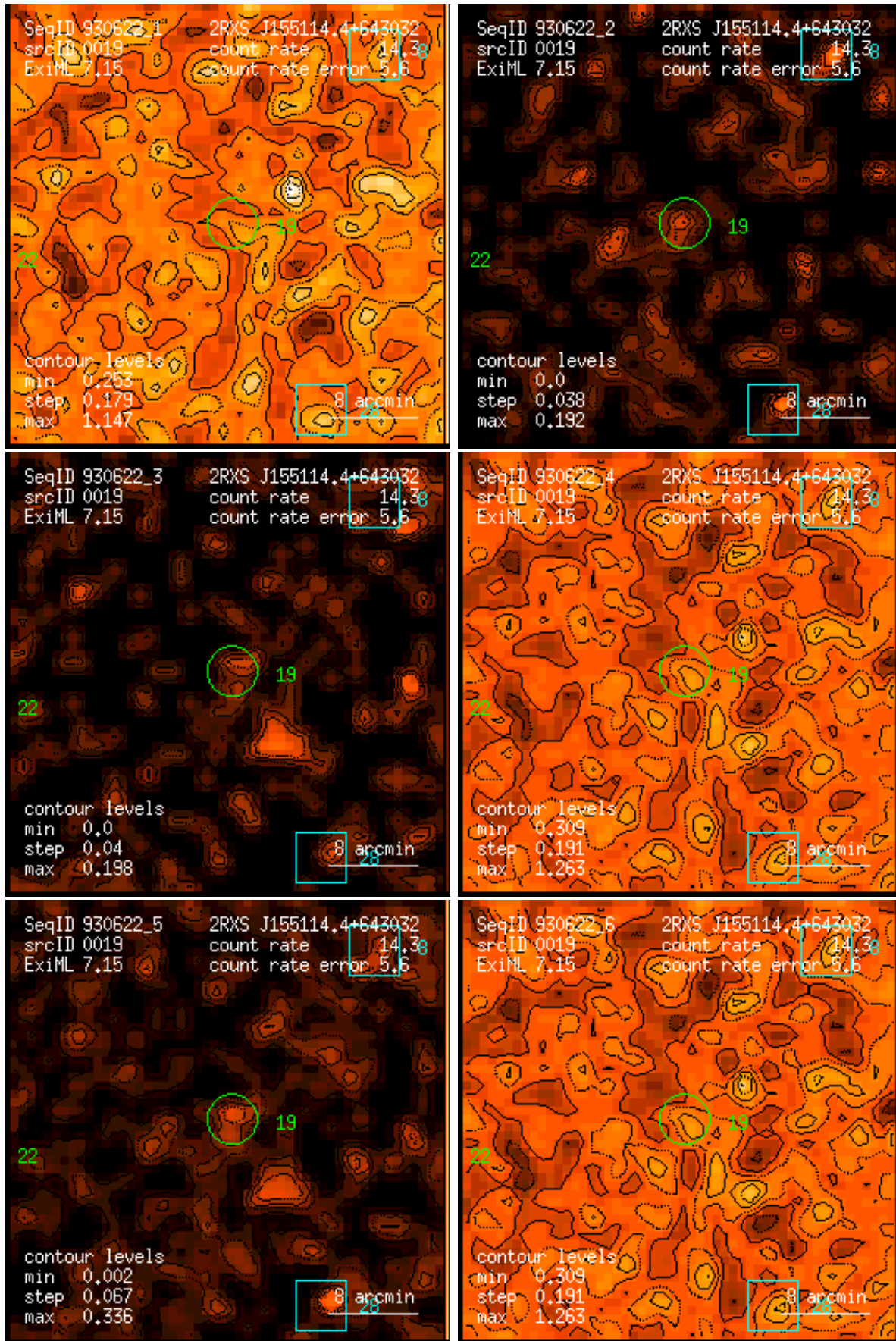
Figure 19: RASS 930622: detection 0019: band rate images, Gaussian filter: (1) PSPC channels 11 – 41, (2) 52 – 90, (3) 91 – 201, (4) 11 – 235, (5) 52 – 201, (6) 11 – 201. Broad band rates in counts/ks. Band rate contour levels in counts/ks/arcmin 2 .
