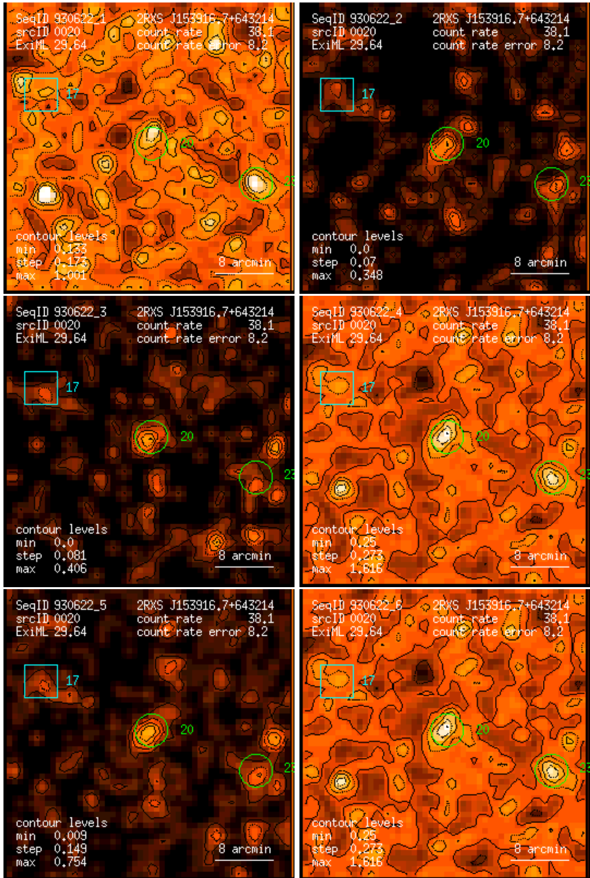
Figure 20: RASS 930622: detection 0020: band rate images, Gaussian filter: (1) PSPC channels 11 – 41, (2) 52 – 90, (3) 91 – 201, (4) 11 – 235, (5) 52 – 201, (6) 11 – 201. Broad band rates in counts/ks. Band rate contour levels in counts/ks/arcmin 2 .
