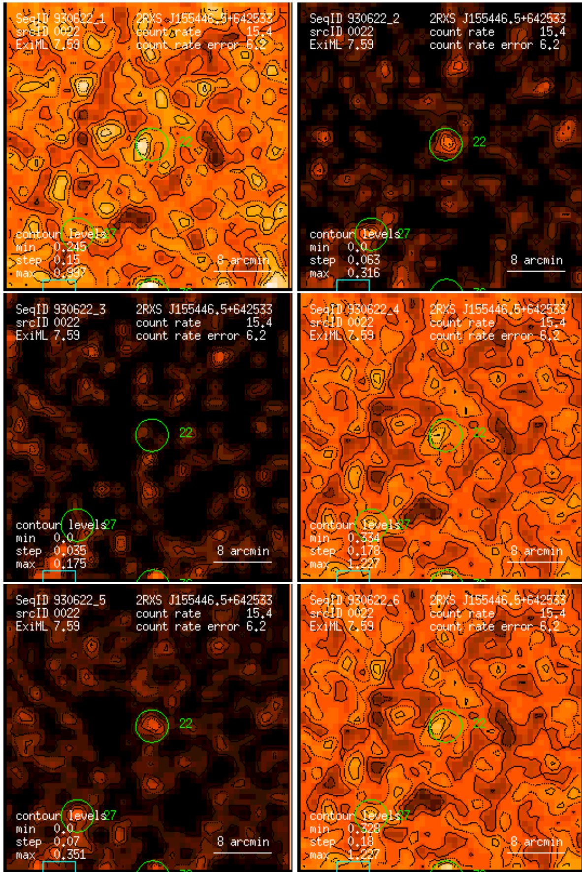
Figure 22: RASS 930622: detection 0022: band rate images, Gaussian filter: (1) PSPC channels 11 – 41, (2) 52 – 90, (3) 91 – 201, (4) 11 – 235, (5) 52 – 201, (6) 11 – 201. Broad band rates in counts/ks. Band rate contour levels in counts/ks/arcmin 2 .
