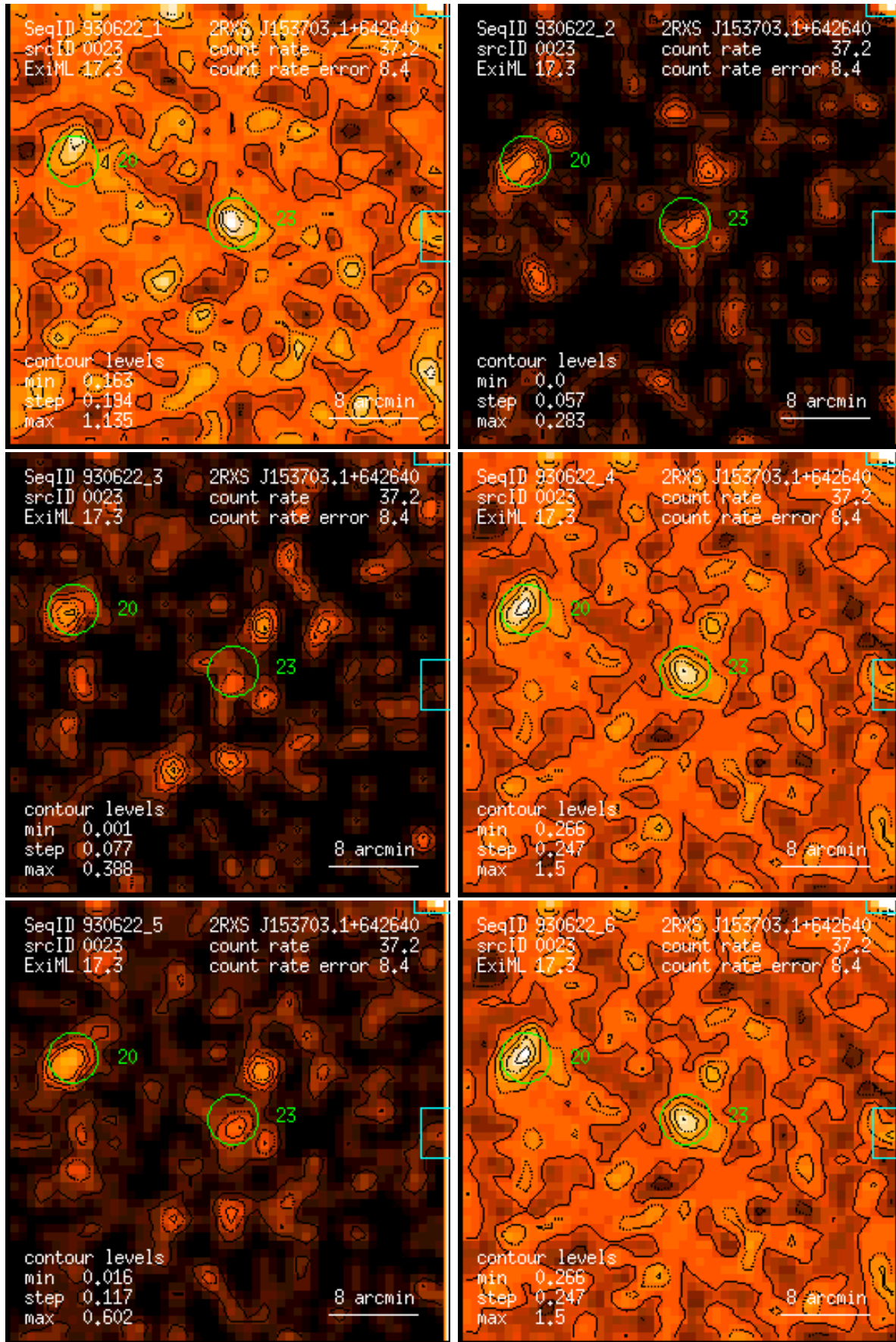
Figure 23: RASS 930622: detection 0023: band rate images, Gaussian filter: (1) PSPC channels 11 – 41, (2) 52 – 90, (3) 91 – 201, (4) 11 – 235, (5) 52 – 201, (6) 11 – 201. Broad band rates in counts/ks. Band rate contour levels in counts/ks/arcmin 2 .
