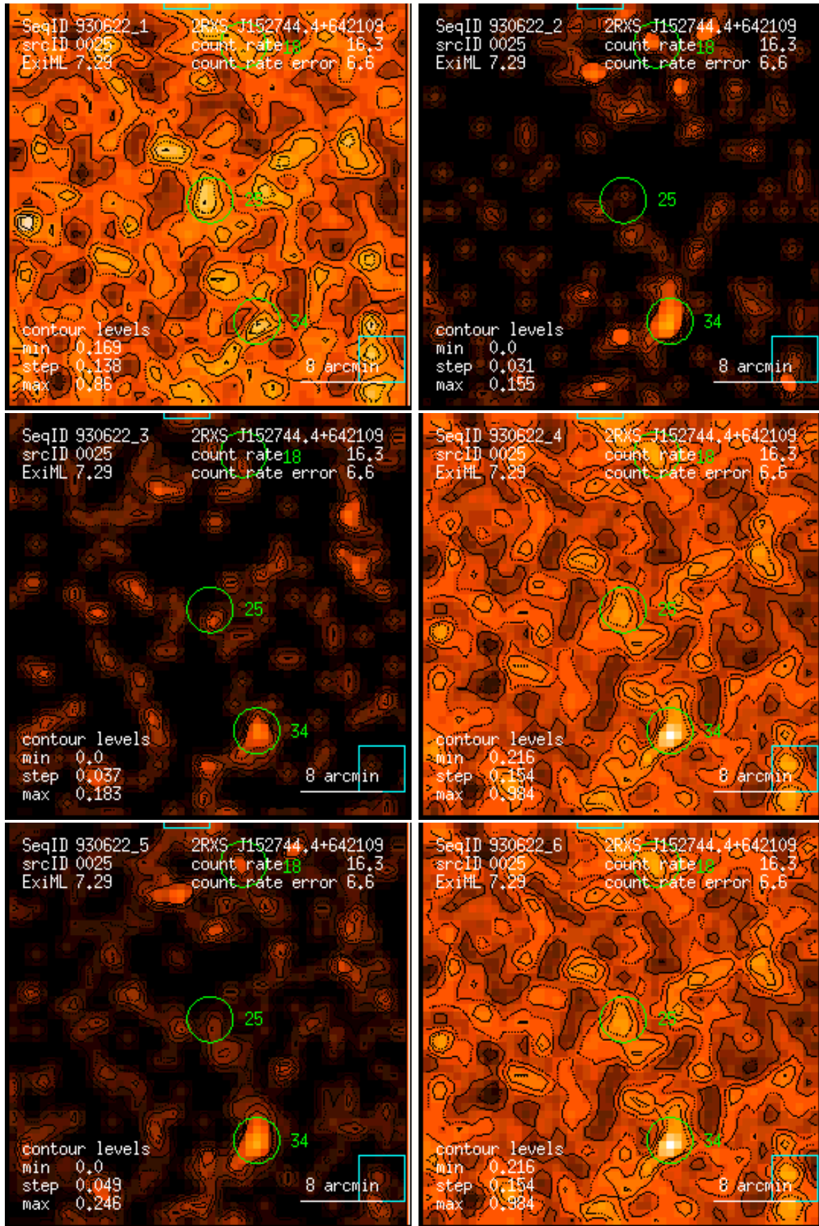
Figure 25: RASS 930622: detection 0025: band rate images, Gaussian filter: (1) PSPC channels 11 – 41, (2) 52 – 90, (3) 91 – 201, (4) 11 – 235, (5) 52 – 201, (6) 11 – 201. Broad band rates in counts/ks. Band rate contour levels in counts/ks/arcmin 2 .
