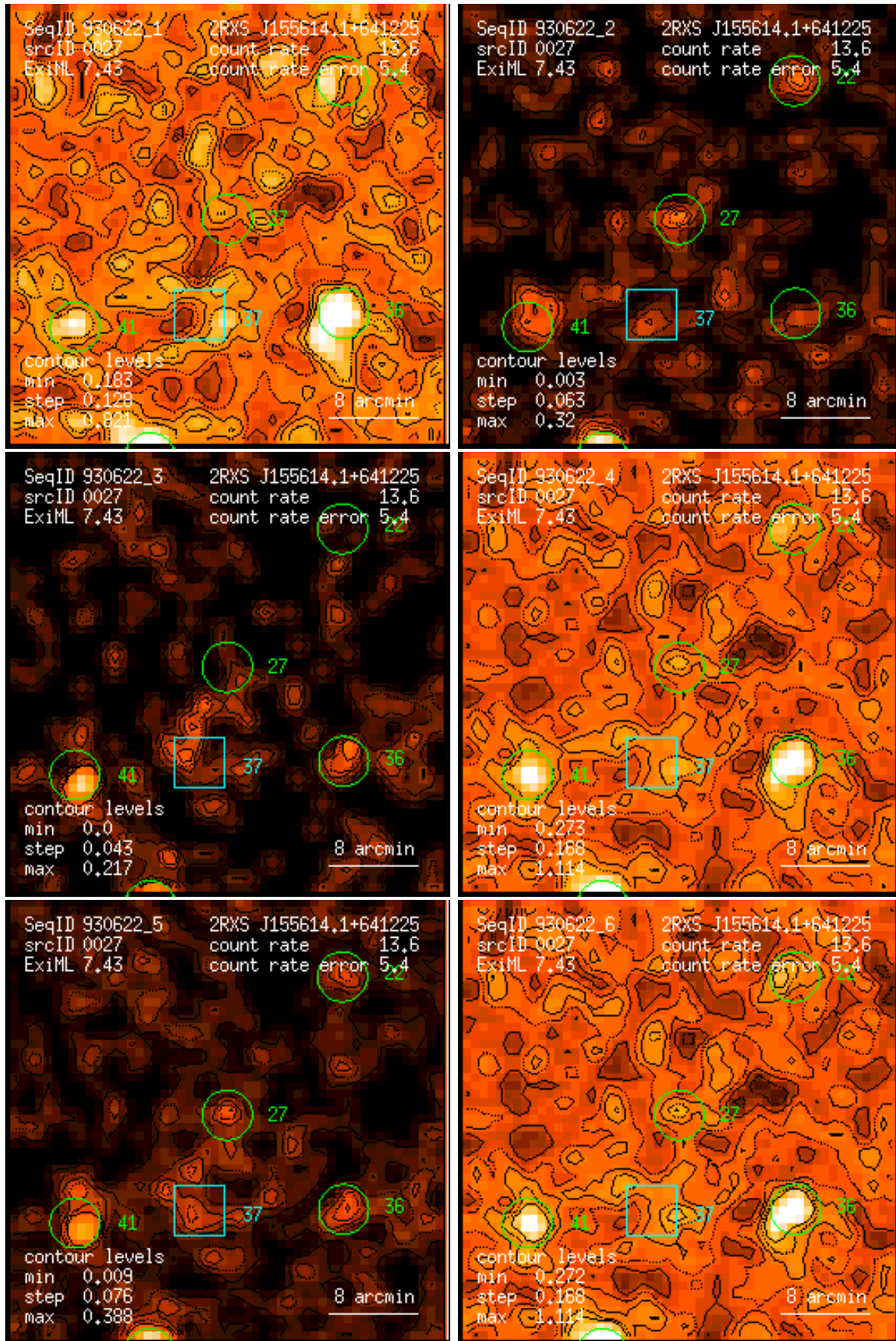
Figure 27: RASS 930622: detection 0027: band rate images, Gaussian filter: (1) PSPC channels 11 – 41, (2) 52 – 90, (3) 91 – 201, (4) 11 – 235, (5) 52 – 201, (6) 11 – 201. Broad band rates in counts/ks. Band rate contour levels in counts/ks/arcmin 2 .
