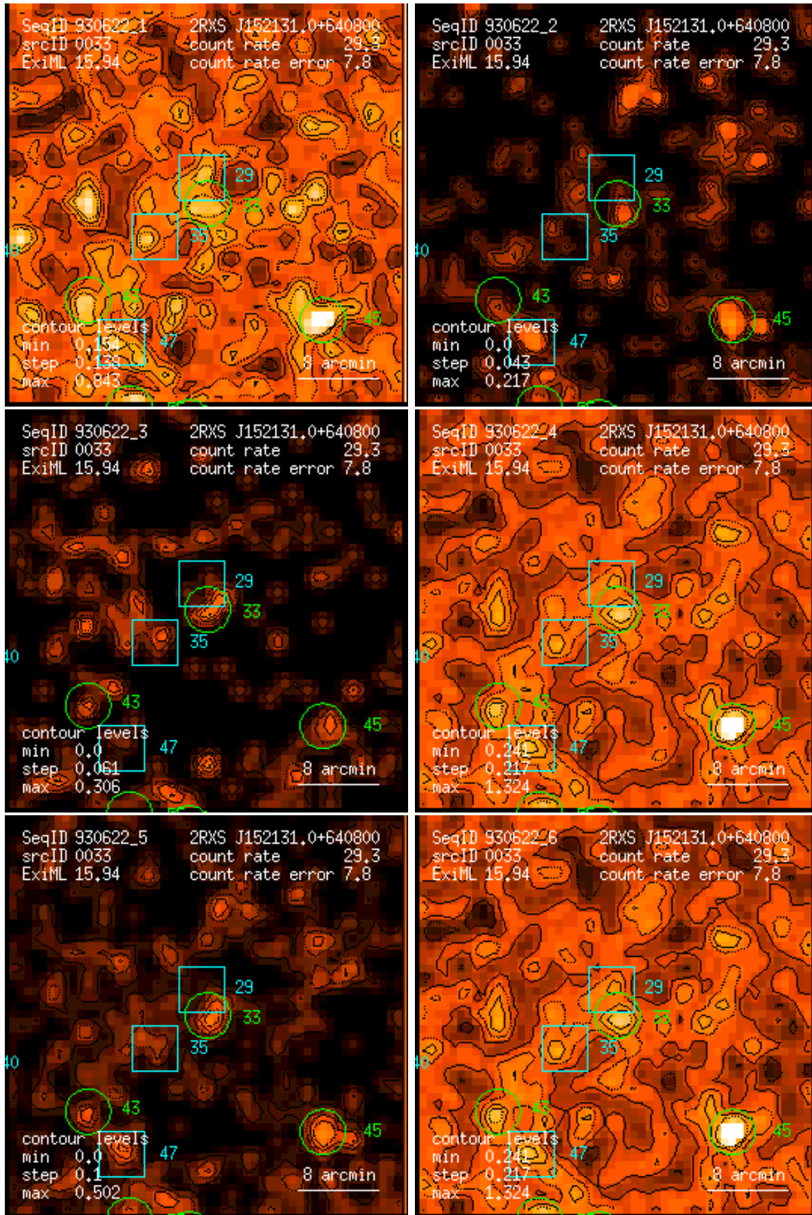
Figure 33: RASS 930622: detection 0033: band rate images, Gaussian filter: (1) PSPC channels 11 – 41, (2) 52 – 90, (3) 91 – 201, (4) 11 – 235, (5) 52 – 201, (6) 11 – 201. Broad band rates in counts/ks. Band rate contour levels in counts/ks/arcmin 2 .
